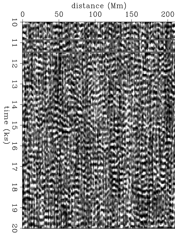
Figure 2: Time-space section through a subset of the raw data.
