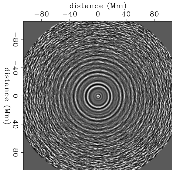
Figure 7: Constant velocity slice through radial transform.
