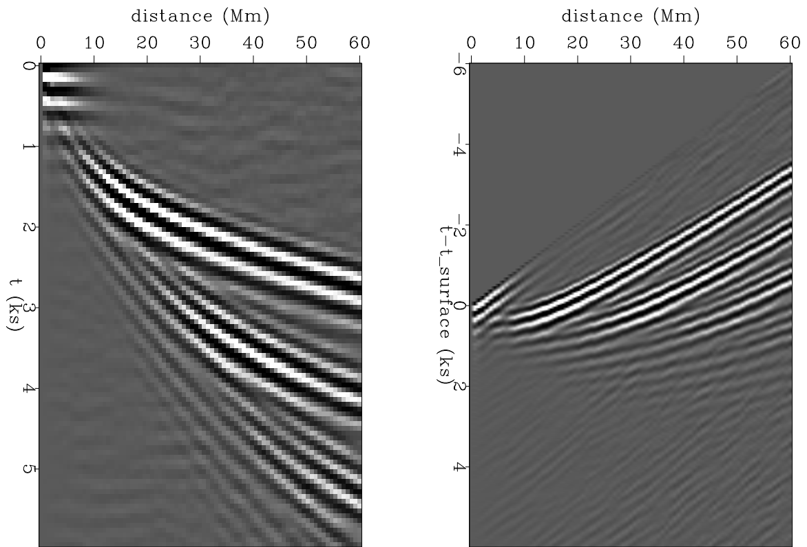
Figure 6: The solar impulse response before (left) and after (right) linear moveout at 10 km/s.
