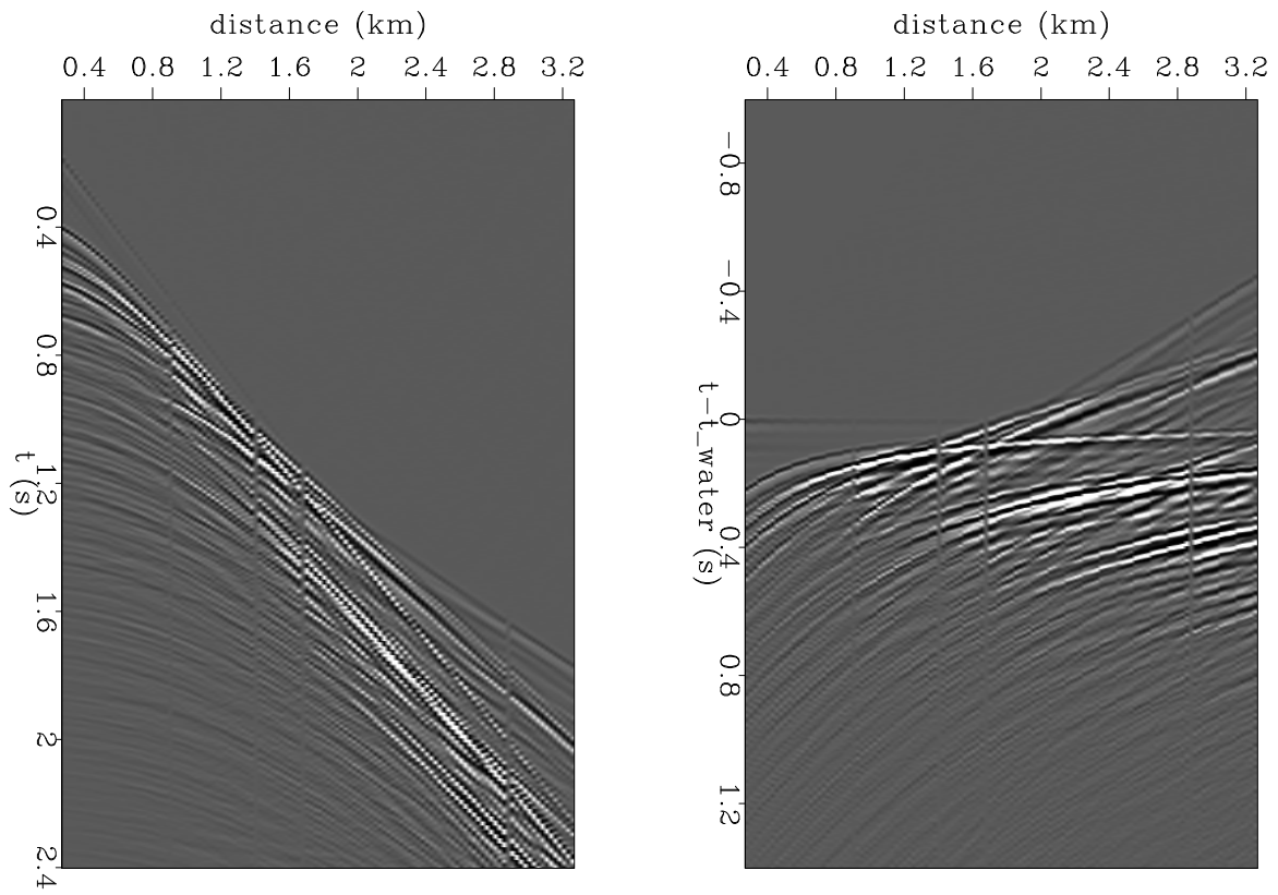
Figure 5: A shot gather from the Gulf of Mexico before (left) and after (right) linear moveout with the water velocity.
