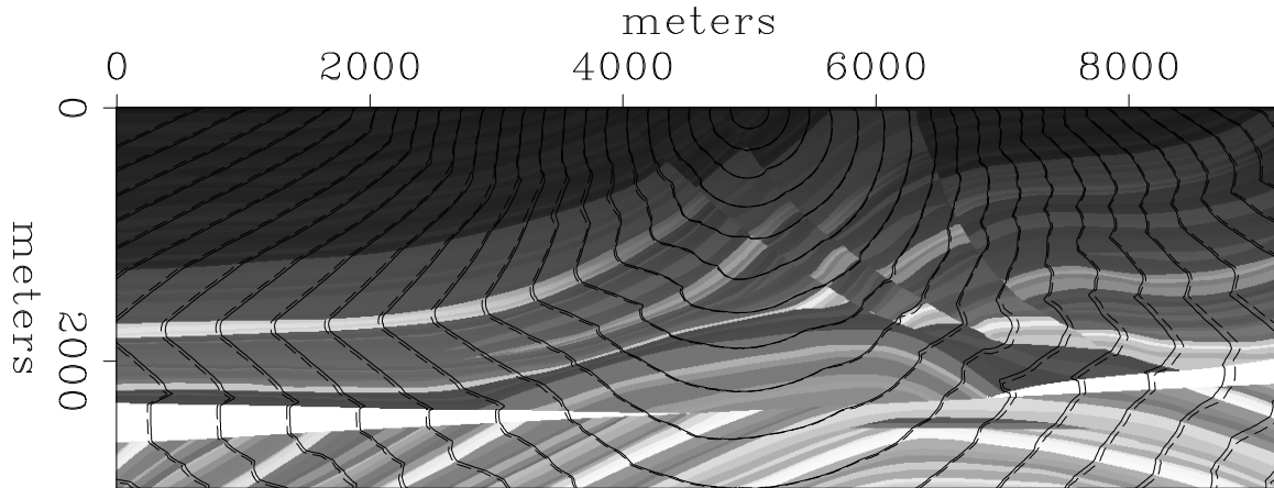
Figure 3: Traveltime contours calculated through the Marmousi velocity model sampled at 4 m. Solid line shows first-order results, and dashed line shows second-order results. James2-marmousi [ER]
