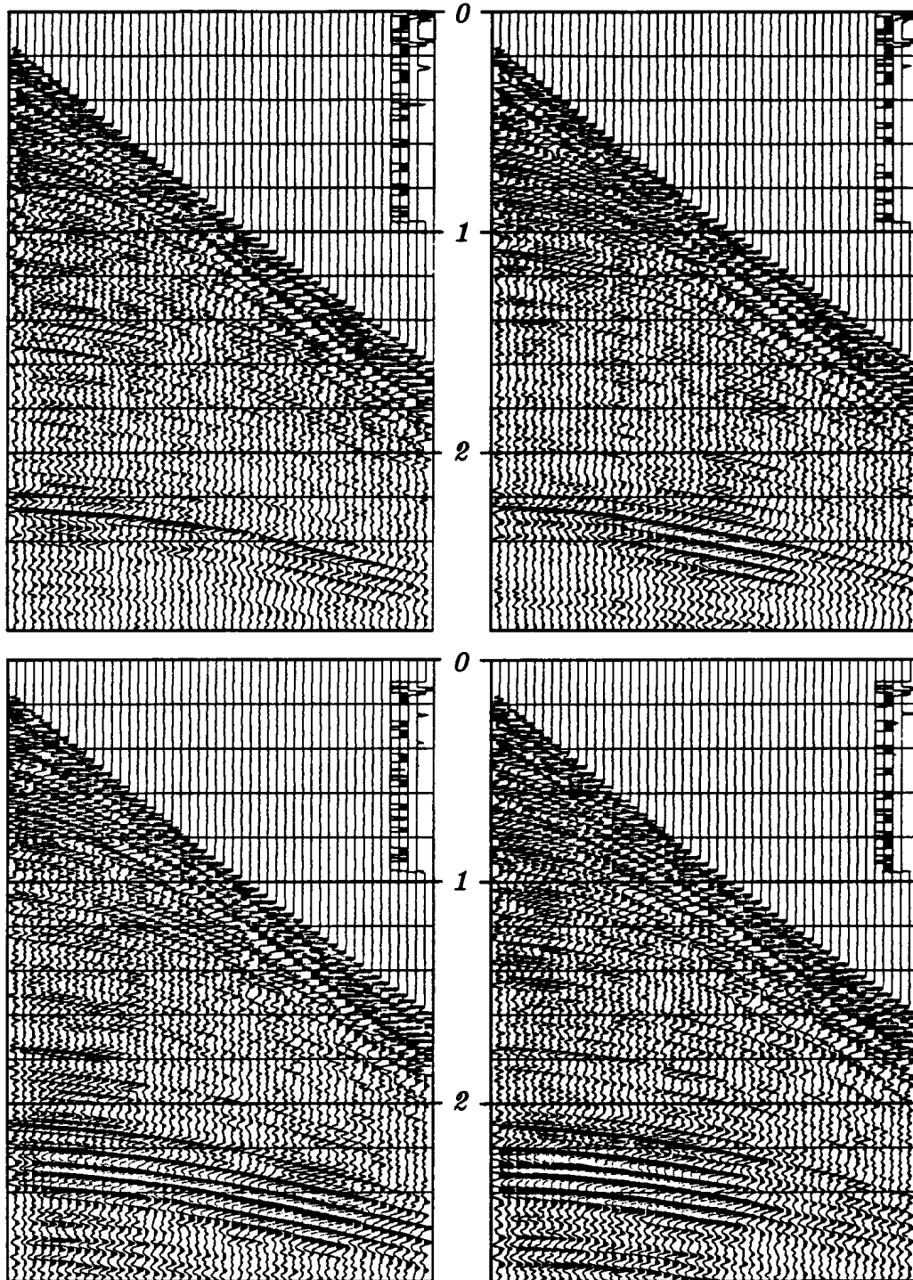
Figure 1: Top left is shot point 210; top right is shot point 220. No processing has been applied to the data except for a display gain proportional to time. Bottom shows shot points 305 and 315. The AVO is too large for realistic layered media models and it changes rapidly from one midpoint to another one nearby. jonl-kjcmg [NR]
