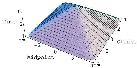
Figure 2: Traveltimes pyramid, composed of common-offset summation curves. sergey1-coffset [CR]
