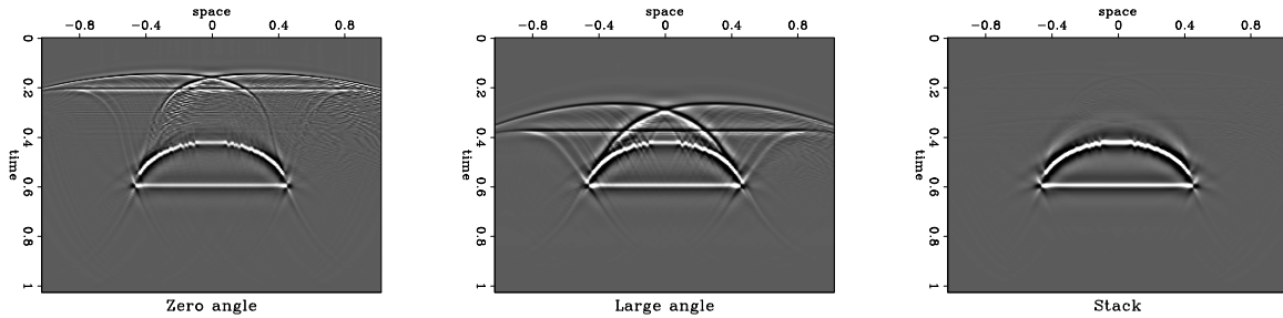
Figure 7: Left: Migrated angle section at small angle. Center: Migrated offset section at large angle. Right: Stack. sergey1-angle.ta.dome [ER]
