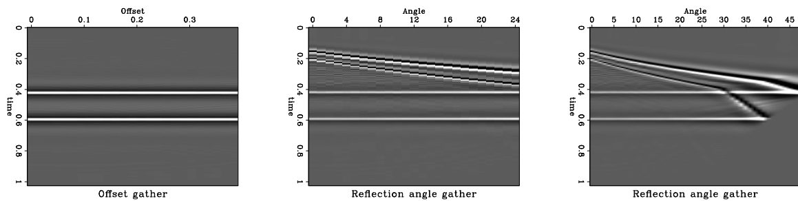
Figure 10: Gathers taken from space location zero in the dome model. Left: Offset domain. Center: Angle domain less than 25^\circ . Right: Angle domain. sergey1-reflect-ta.dome [ER]
