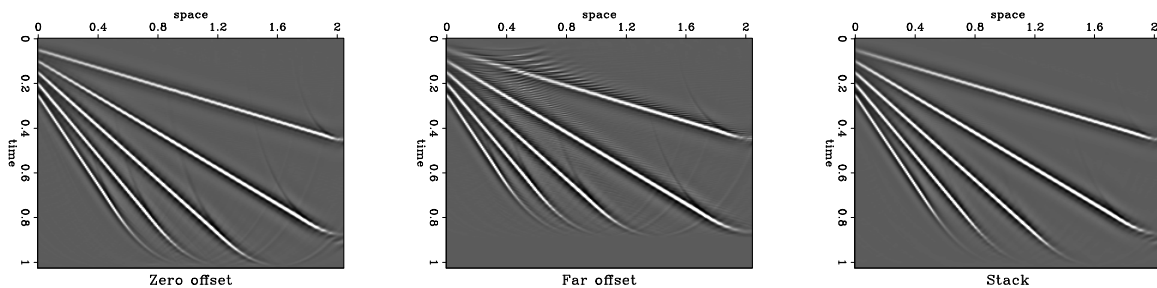
Figure 8: Left: Migrated offset section at zero offset. Center: Migrated offset section at far offset. Right: Stack. sergey1-offset.lines [ER]
