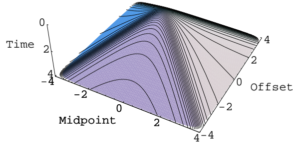
Figure 3: Traveltime pyramid, composed of common-reflection-angle summation curves. sergeyl-cangle [CR]
