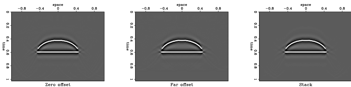
Figure 6: Left: Migrated offset section at zero offset. Center: Migrated offset section at far offset. Right: Stack. sergey1-offset.dome [ER]
