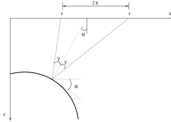
Figure 1: Reflection rays in a constant-velocity medium: a scheme. sergey1-rays [NR]
