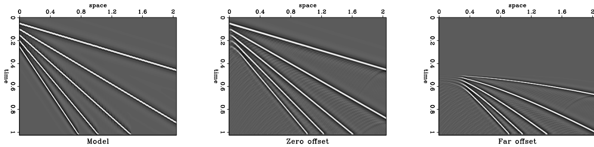
Figure 5: Left: Model. Center: Data at zero offset. Right: Data at far offset. sergey1-data.lines [ER]
