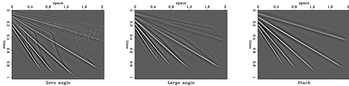
Figure 9: Left: Migrated angle section at zero angle. Center: Migrated angle section at large angle. Right: Stack. sergey1-angle-ta.lines [ER]
