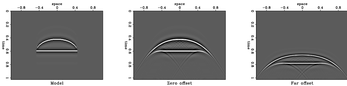
Figure 4: Left: Model. Center: Data at zero offset. Right: Data at far offset. sergey1-data.dome [ER]
