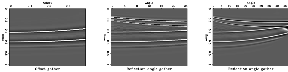
Figure 11: Gathers taken from space location zero in the dome model and migrated at too low a velocity. Left: Offset domain. Center: Angle domain less than 25^\circ . Right: Angle domain. sergey1-reflect-ta.fast.dome [ER]
