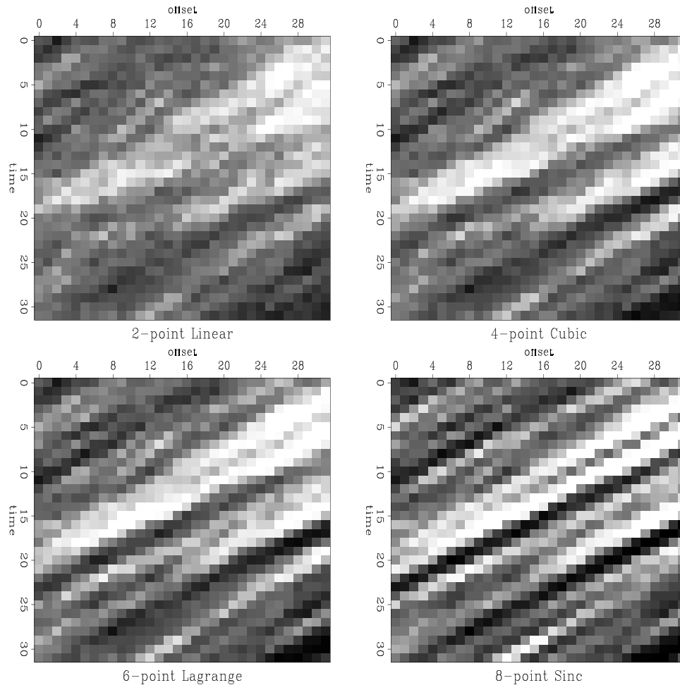
Figure 4: Interpolation schemes compared. Deconvolution of random image with labeled steering filters. morgan2-interp-comp [ER]
