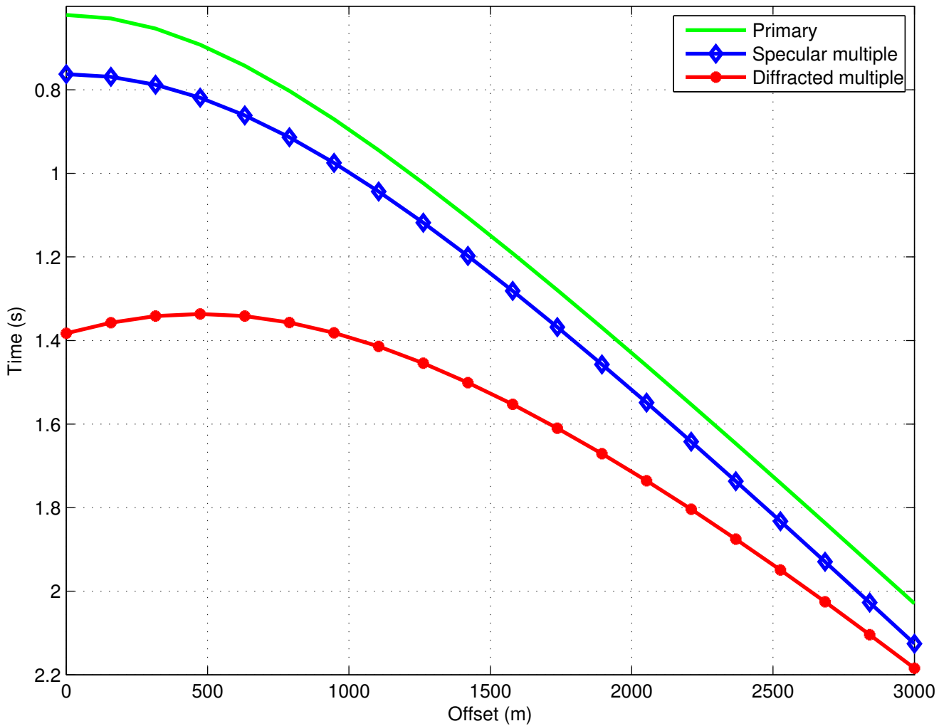
CMP gather
