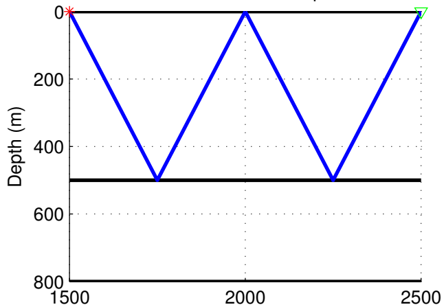
Water-bottom multiple
