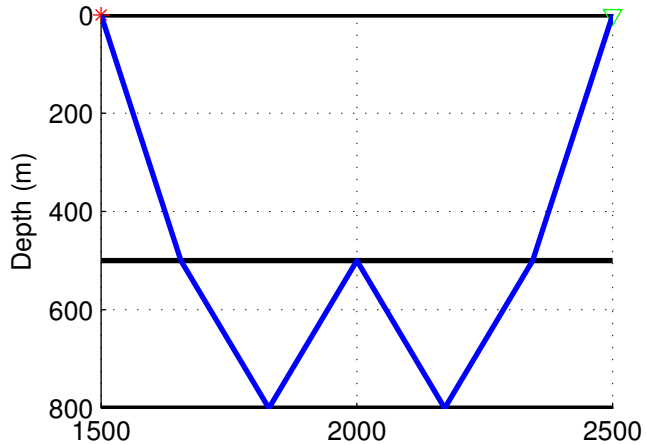
Internal multiple
