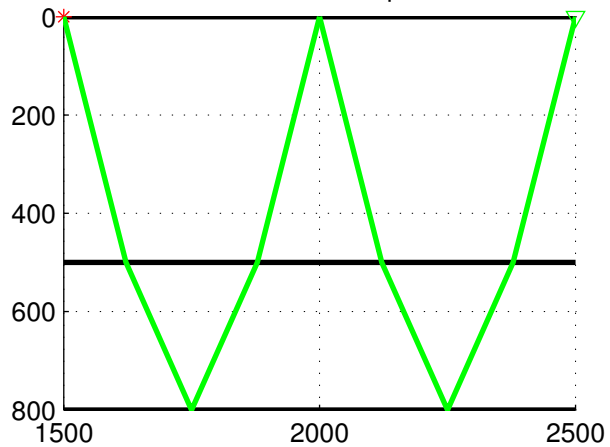
Reflector multiple
