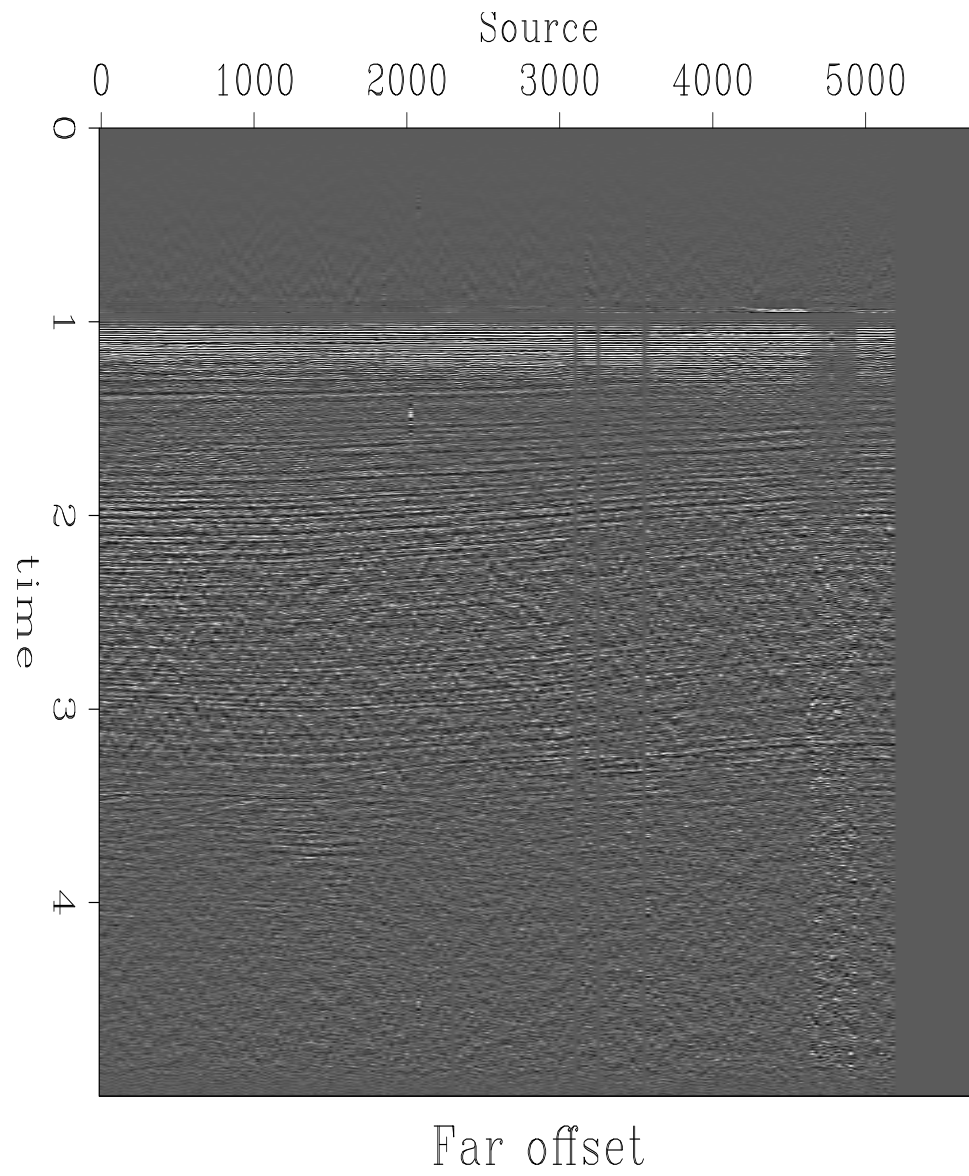
Figure 3: Far offset gather adriatic-sea-far-offset [ER]
