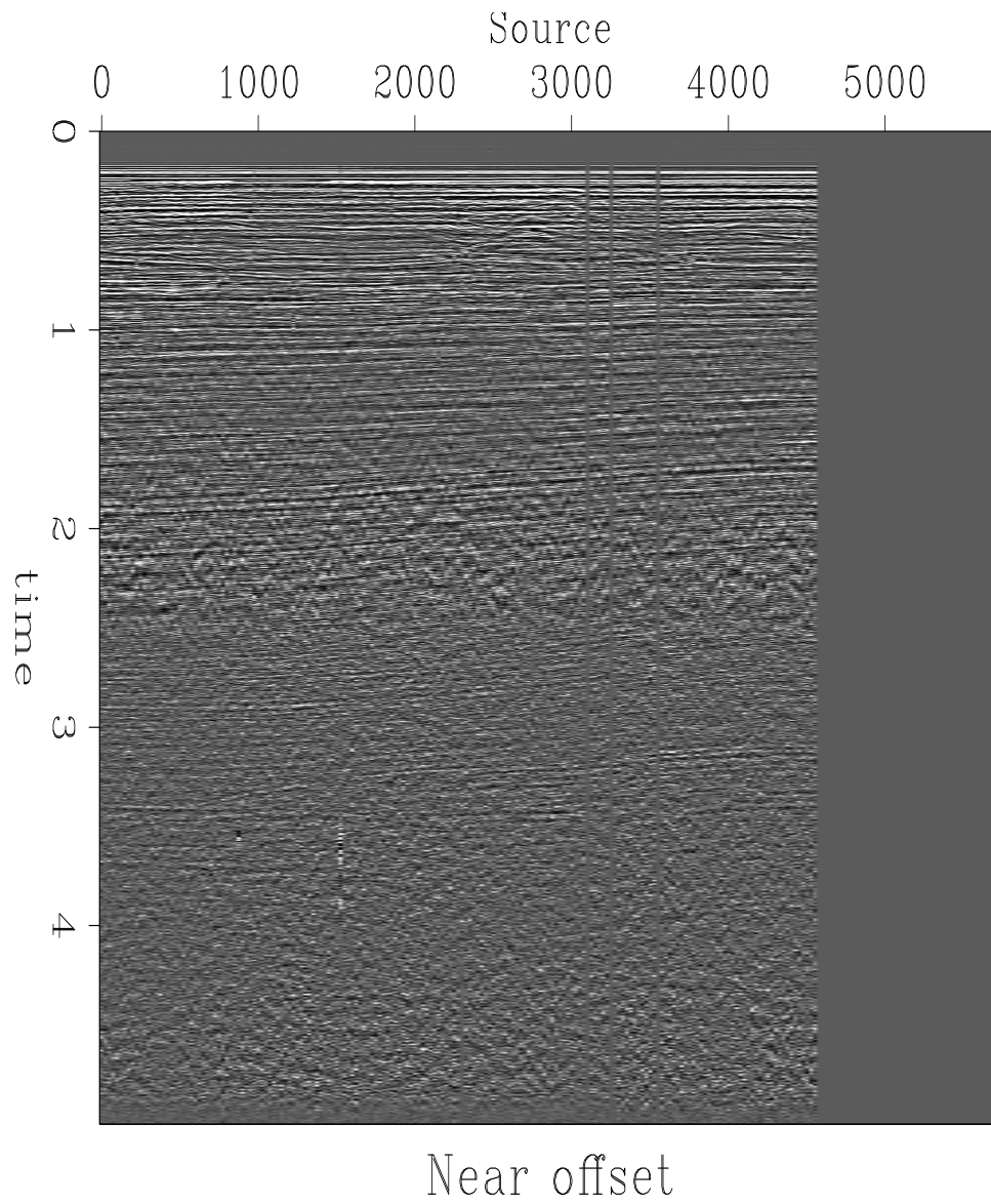
Figure 2: Near offset gather adriatic-sea-near-offset [ER]
