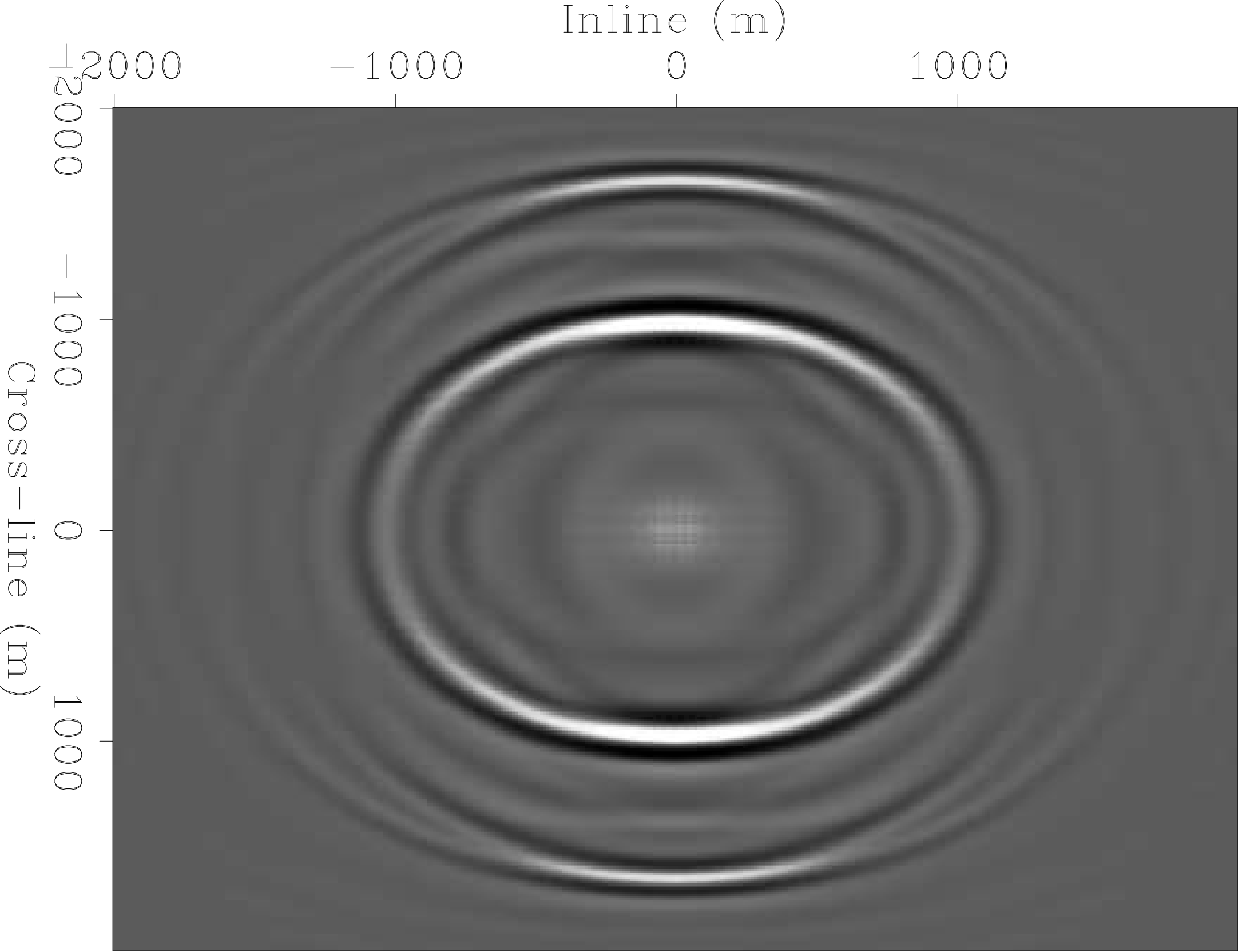
Depth Slice @ 1100 m
