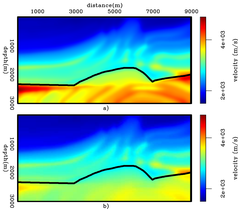
Figure 6: Velocity models for in the Marmousi example: a) Smooth velocity model used to model the Born data. b) Background velocity model used to migrate the Born data, and to model and migrate PERM data.
