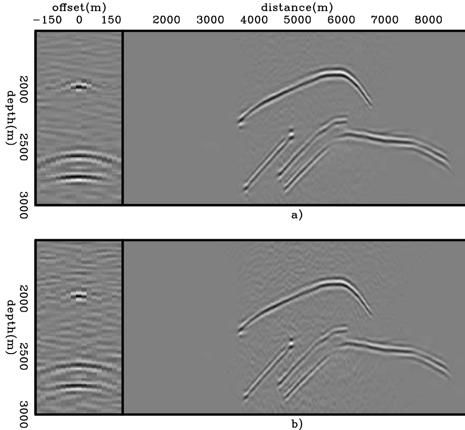
Figure 12: Pre-stack images computed with: a) Four random realizations of ISPEW, and b) a single random realization.
