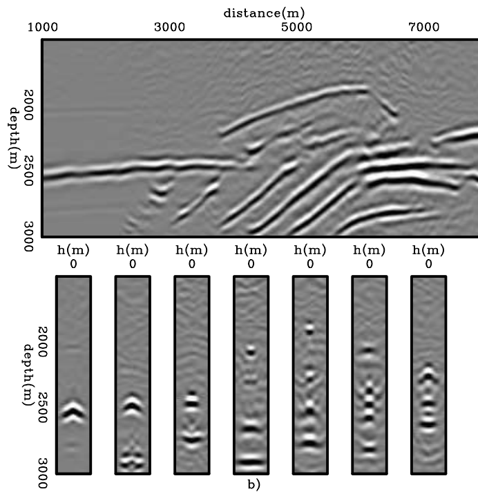
Figure 4.14: a) Initial and b) final background image for the optimization with 35 ISPEWs. mvags/.ismarm301
