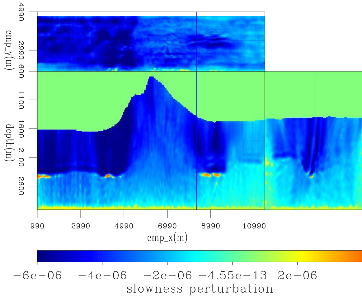
Figure 5.14: Slowness perturbation without smoothing and extracting the signed fourth root of the gradient. 3dex/. 3dex211
