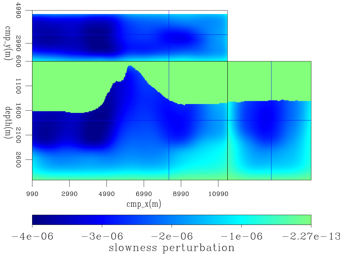
Figure 5.15: Slowness perturbation after B-spline smoothing the slowness perturbation of Figure 5.14. 3dex/. 3dex212
