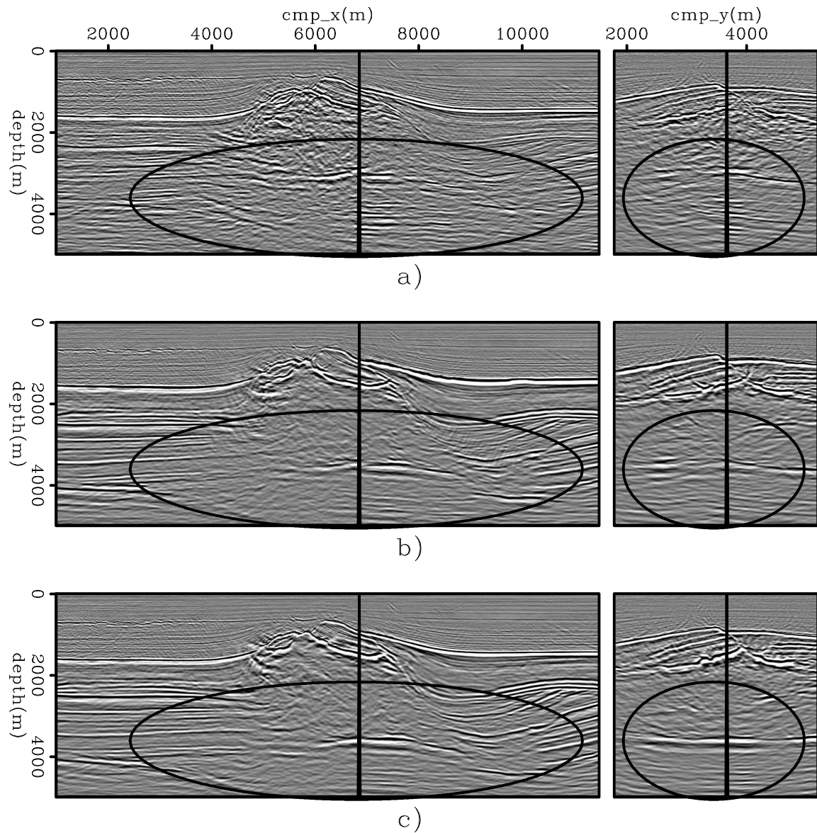
Figure 5.35: On the left panel is the in-line 3680 and on the right panel is the cross-line 6880 of the CAM images obtained with: a) the initial velocity model, b) the original velocity model, and c) the final velocity model after optimization for the chalk layer, salt flooding, and sub-salt velocity optimization. The oval in the in-line of the final image shows better focusing and continuity for the sub-salt reflectors. Besides focusing and continuity, the oval in the cross-line of the final image shows unstructured sub-salt reflectors not pulled up by velocity errors. 3dex/. 3dex501
