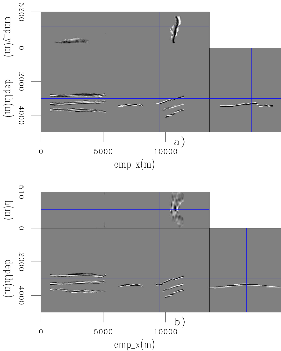
Figure 5.28: Slices through the windowed prestack image, showing the selected reflectors for the modeling of 30 3D ISPEWs to be used in the sub-salt velocity optimization: a) the zero subsurface offset, and b) the in-line 3520. 3dex/. 3dex401
