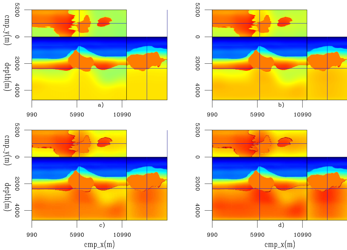
Figure 5.30: Slices through velocity models for: a) first iteration, b) third iteration, c) fifth iteration, and d) seventh iteration. 3dex/. 3dex403
