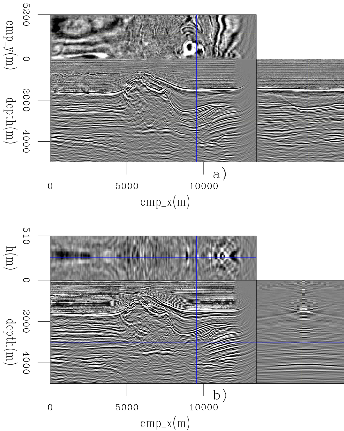
Figure 5.27: Slices through the prestack image computed with the migration velocity of Figure 5.25: a) the zero subsurface offset, and b) the in-line 3520. 3dex/. 3dex400
