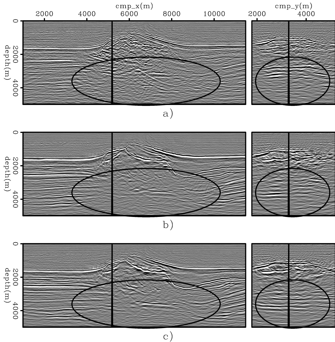
Figure 5.34: On the left panel is the in-line 3320 and on the right panel is the cross-line 5220 of the CAM images obtained with: a) the initial velocity model, b) the original velocity model, and c) the final velocity model after optimization for the chalk layer, salt flooding, and sub-salt velocity optimization. The oval in the in-line of the final image show better focusing and continuity for the sub-salt reflectors as well as for the salt flank. Besides focusing and continuity, the oval in the cross-line of the final image show unstructured sub-salt reflectors not pulled up by velocity errors.
