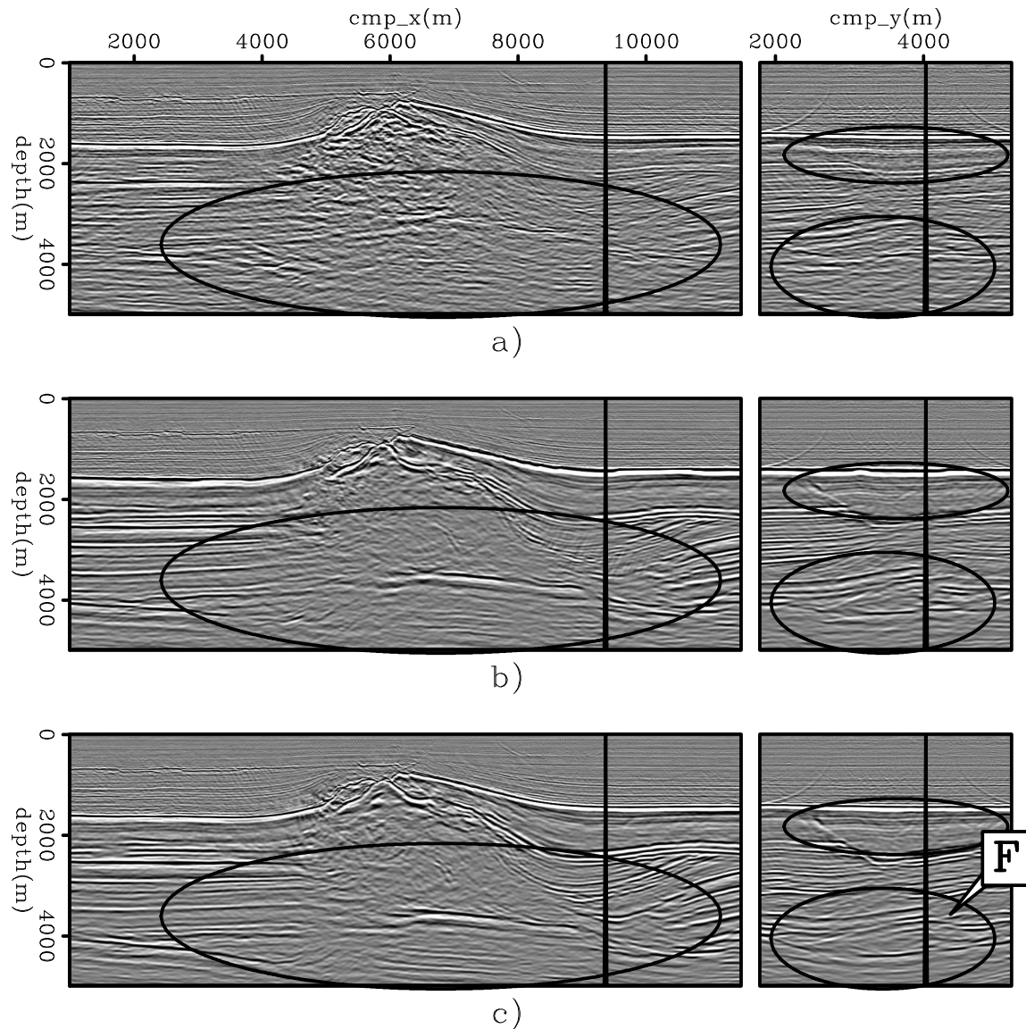
Figure 5.36: On the left panel is the in-line 4060 and on the right panel is the cross-line 9400 of the CAM images obtained with: a) the initial velocity model, b) the original velocity model, and c) the final velocity model after optimization for the chalk layer, salt flooding, and sub-salt velocity optimization. The oval in the in-line of the final image show better focusing and continuity for the sub-salt reflectors. In the cross-line, the upper oval of the final image show better definition of subtle faults in the chalk layer, the lower oval highlights better continuity of the reflectors, and the arrow labeled "F" indicates better fault imaging not clear in the initial and original images.
