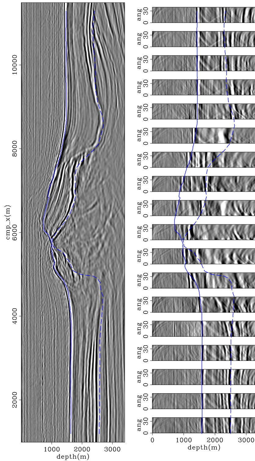
Figure 5.22: In-line 3180 of the CAM image with the optimized velocity model of Figure 5.20. On the left is the zero-subsurface offset section, and on the right ADCIGs. Notice flatter reflectors in the ADCIGs compared to those in Figure 5.10. The continuous blue line is the top of chalk, and the dashed blue line it the base of chalk.
