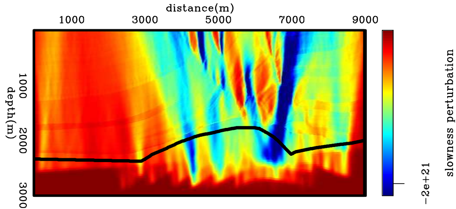
Figure 4.12: Slowness perturbation from back-projected image perturbations computed with 35 ISPEWs. mvags/.ismarm206
