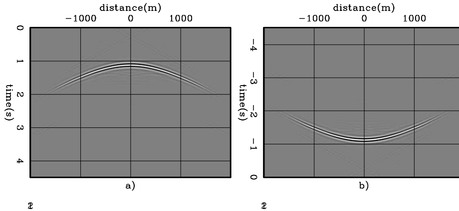
Figure 2.12: Data synthesized by PERM having as the initial condition the dipping reflector in the SODCIG at x_m = 0 m. a) The receiver wavefield. b) The source wavefield. perm/. dip02
