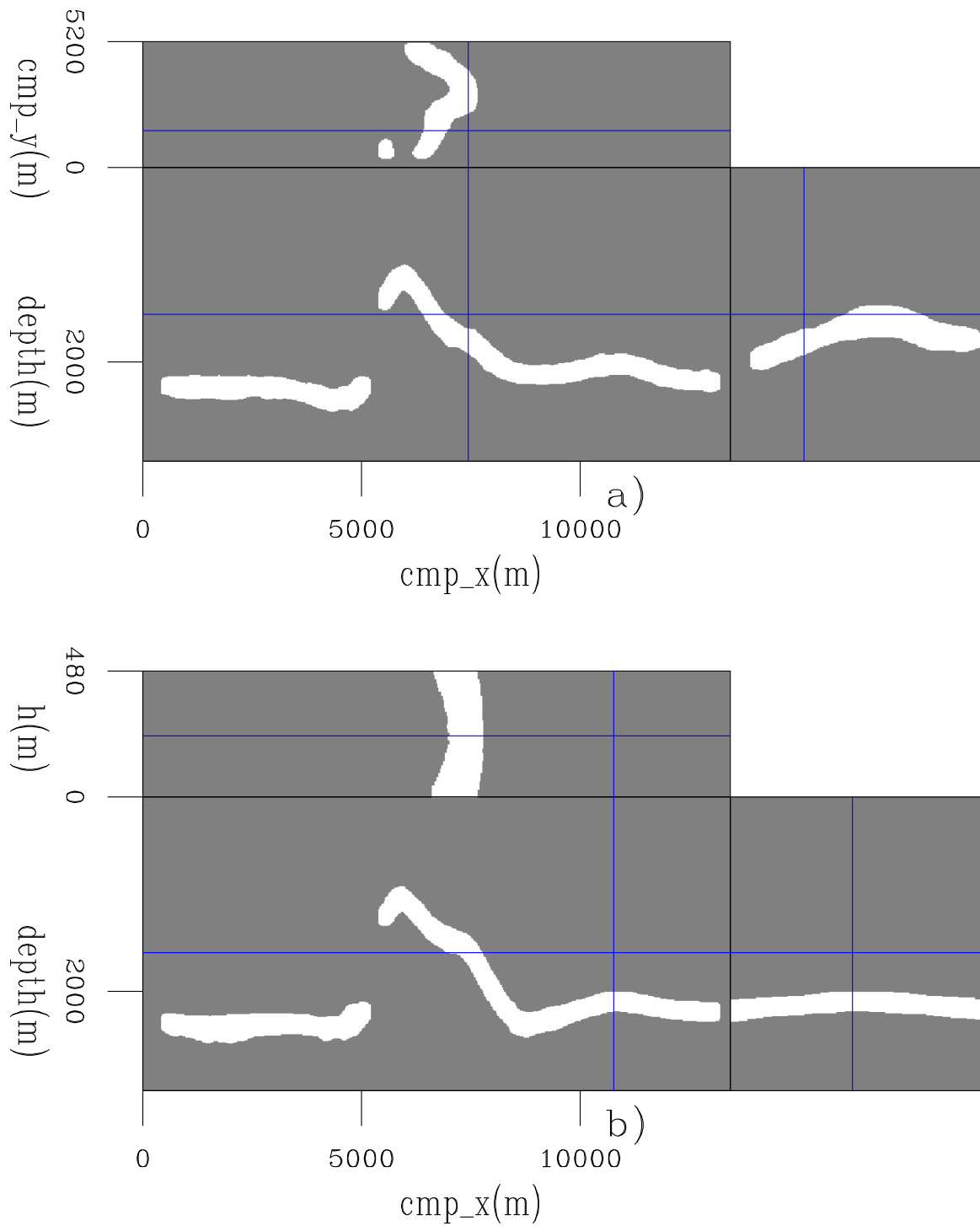
Figure 5.11: Slices through the prestack-mask operator to select the base of chalk, showing: a) the zero subsurface offset, and b) the in-line 3520. 3dex/. 3dex106a
