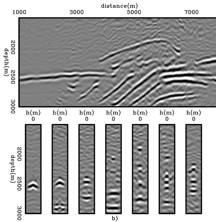
Figure 4.13: a) Initial and b) final background image for the optimization with 11 ISPEWs. mvags/.ismarm302
