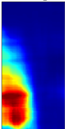
15th off-diagonal
