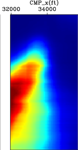
main diagonal
