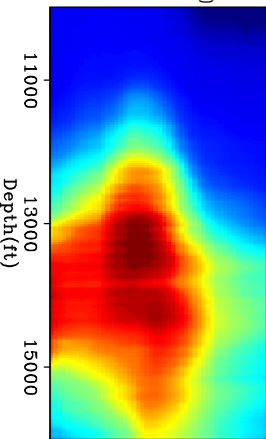
5th off-diagonal
