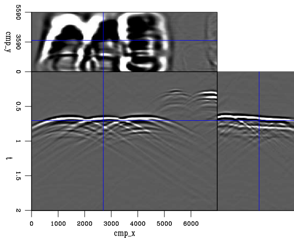
Figure 7: PERM receiver wavefield of one areal shot.
