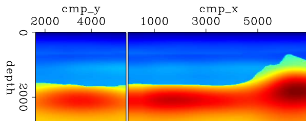
Figure 8: Optimized velocity model. Left: cross-line at 3500 m. Right: in-line at 3760 m.
