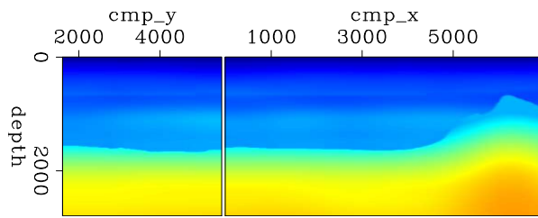
Figure 5: Initial velocity model. Left: cross-line at 3500 m. Right: in-line at 3760 m.
