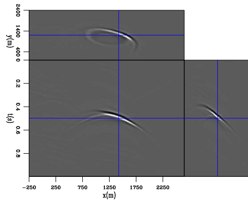
Figure 3: 3D-PERM receiver wavefield. The left panel is the in-line at y = 1200 m, the right panel is the cross-line at x = 1400 m, and the top panel is the time-slice at t = 0.5 s.
