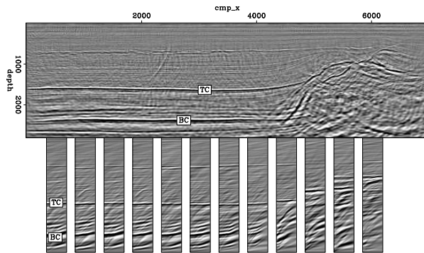
Figure 6: Angle-gathers after CAM with the initial velocity. Top: zero-angle section. Bottom: ACDCIGs selected roughly at the same x position in the section above.
