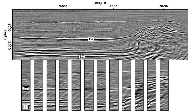
Figure 9: Angle-gathers after CAM with the optimized velocity. Top: zero-angle section. Bottom: ACDCIGs selected roughly at the same x position in the section above.
