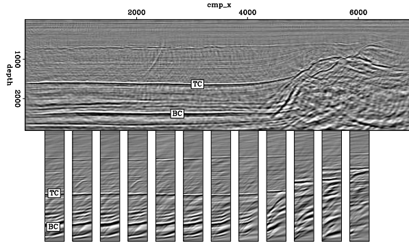
Figure 6: Angle-gathers after CAM with the initial velocity. Top: zero-angle section. Bottom: ACDCIGs selected roughly at the same x position in the section above.
