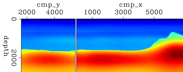
Figure 8: Optimized velocity model. Left: cross-line at 3500 m. Right: in-line at 3760 m.
