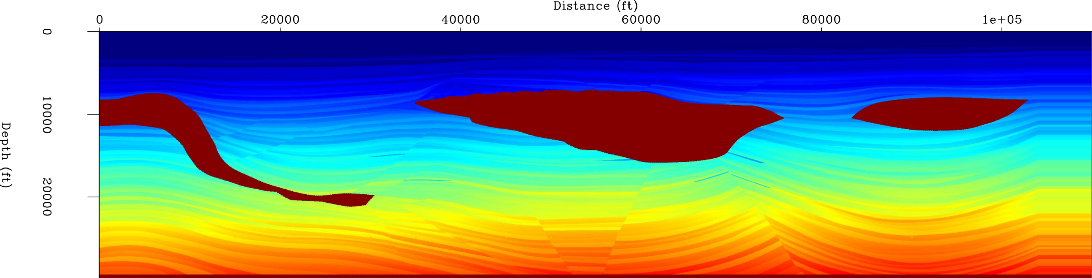
Pluto - P-wave Velocity
