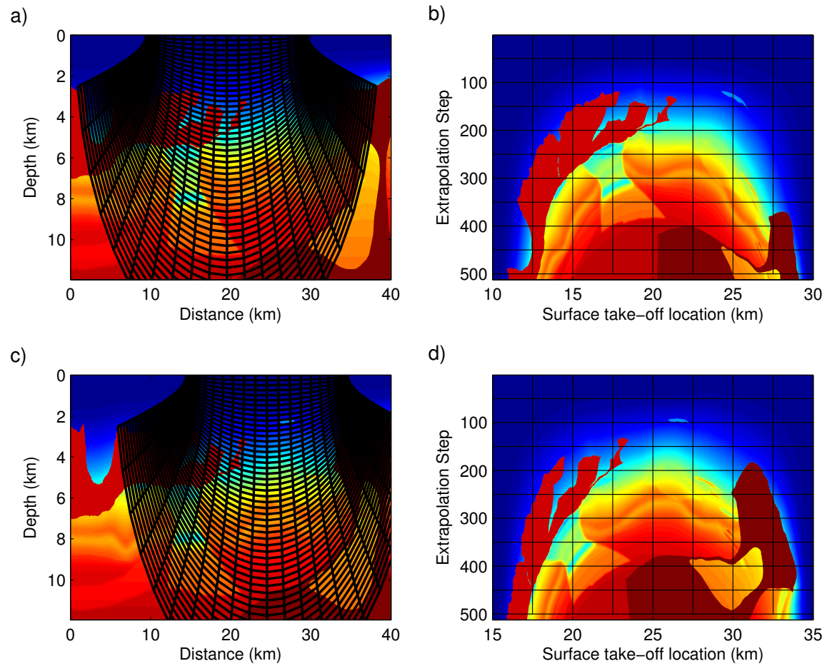
Figure 2: Prestack migration test in elliptic coordinates. a) Benchmark synthetic velocity model with an overlying elliptic coordinate system. b) Effective slowness model in the transformed elliptic coordinate system in a). c) Benchmark synthetic velocity model with a different overlying elliptic coordinate system. d) Effective elliptic coordinate slowness model for the coordinate system in c).
