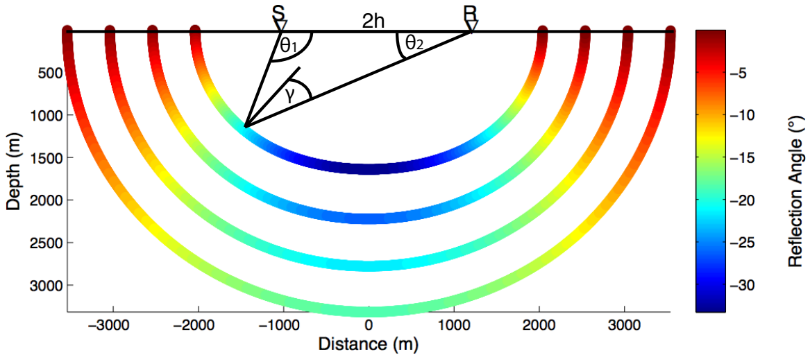
Figure 4: Theoretical results for an elliptic isochron for four travel times in a constant velocity medium. The elliptic surfaces are color-coded according to reflection opening angle.
