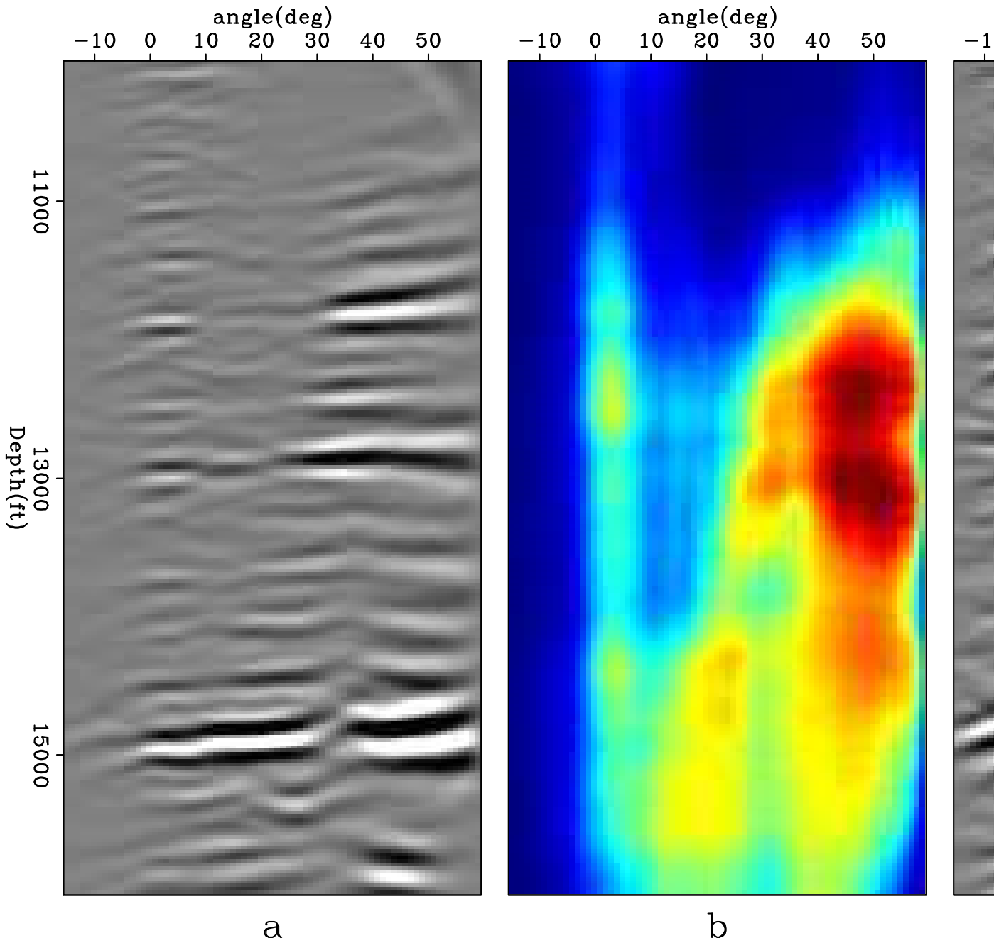
Figure 4: ADCIGs and diagonal of the transformed angle-domain Hessian at CMP coordinate 33200 ft. Before amplitude compensation (a); diagonal of the Hessian in the angle domain (b); and after amplitude compensation (c). Note the improved amplitude balance in the angle direction. join16 [ER]
