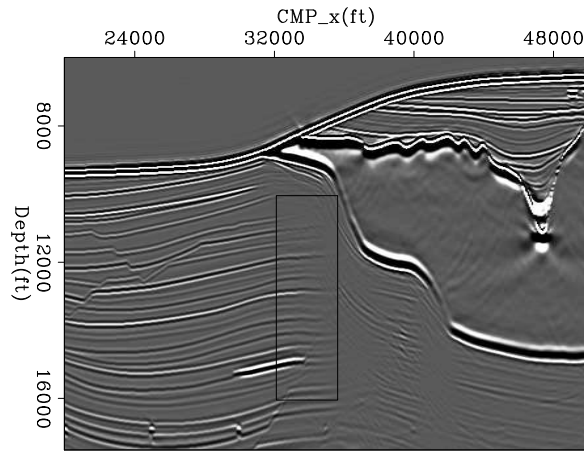
Figure 1: Shot profile migration of part of Sigsbee dataset — zero-subsurface offset. The small box highlights the target area. Sigsbee [ER]
