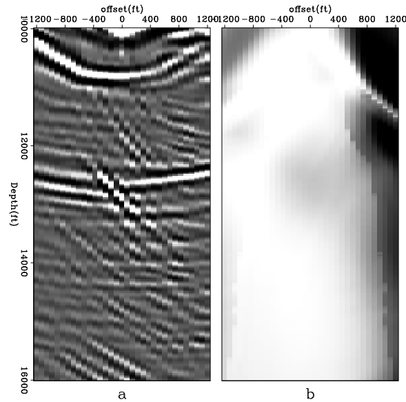
Figure 3: SODCIG and diagonal of the subsurface-offset Hessian at CMP coordinate 33200 ft. Upward curved events correspond to multiples. Note the effects of poor illumination represented by horizontal and dipping straight events in the SODCIG. Ojoin50 [ER]
