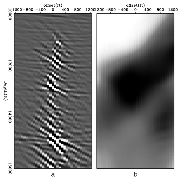
Figure 2: SODCIG and diagonal of the subsurface-offset Hessian at CMP coordinate 33200 ft. Note the effects of poor illumination represented by horizontal and dipping straight events in the SODCIG. Ojoin16 [ER]
