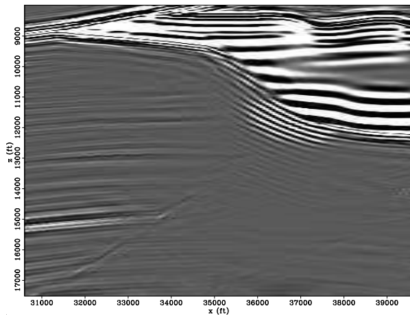
Figure 8: Residuals of the inversion in the poststack image domain with a filtered migration as the input after seven iterations.
