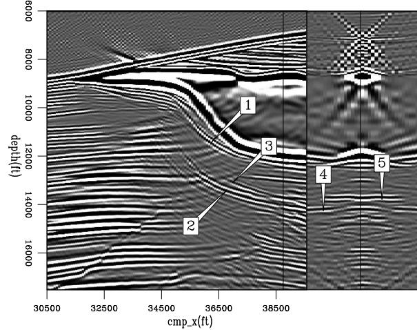
Figure 2: Sigsbee2B shot-profile migration. 1) 1^{st} -order peg-leg diffracted multiples; 2) 1^{st} -order peg-leg multiple from the base of the salt; 3) internal multiples originated at the salt limits; 4) 1^{st} -order peg-leg multiple from the base of the salt; and, 5) internal multiples originated at the salt limits. The front face corresponds to the image at zero subsurface-offset, and the side face corresponds to the subsurface-offset gather at x = 38600 ft.
