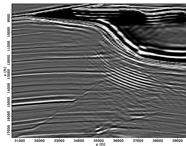
Figure 5: Inversion in the poststack image domain with the unfiltered migration as the input (equation 3) after seven iterations of a conjugate-gradient iterative solver and no regularization.
