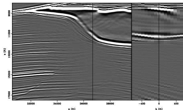
Figure 4: Sigsbee2b shot-profile migration (subsurface-offset), after multiple attenuation. The front face corresponds to the image at zero subsurface-offset, and the side face corresponds to the subsurface-offset gather at x = 36800 ft. Compare with Figure 3.
