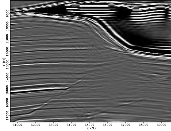
Figure 6: Inversion in the poststack image domain with a filtered migration as the input to equation 3.
