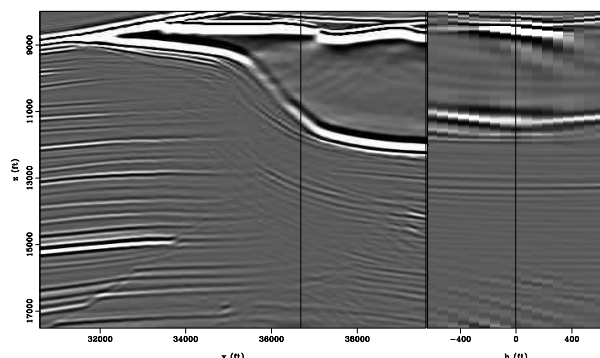
Figure 3: Sigsbee2b shot-profile migration (subsurface-offset). The front face corresponds to the image at zero subsurface-offset, and the side face corresponds to the subsurface-offset gather at x = 36800 ft. Poorly illuminated areas are dominated by the presence of migrated multiples.
