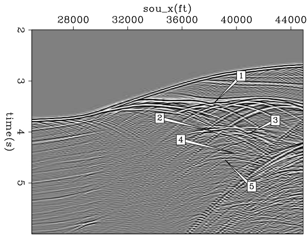
Figure 1: Sigsbee2B zero-offset time section. The labels correspond to 1) top of the salt; 2) base of the salt; 3) 1^{st} -order peg-leg diffracted multiples; 4) internal multiples originated at the salt limits; and, 5) 1^{st} -order peg-leg multiple from the base of the salt.
