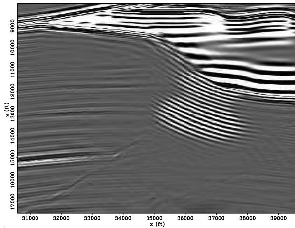
Figure 7: Residuals of the inversion in the poststack image domain with the unfiltered migration as the input after seven iterations.
