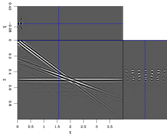
Figure 6: ] Areal shot migration of 11 sets, each set containing the summation of areal shots initiated at every 11 th SODCIG. Original figure was substituted.[ER] armig11W [ER]
