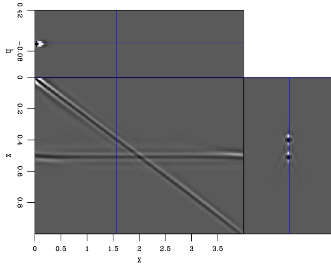
Figure 1: ] Prestack cube obtained with shot profile migration with the correct velocity. [ER] mig08 [ER]
