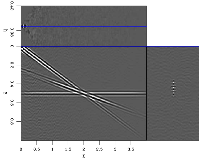
Figure 12: ] Areal shot migration of randomly encoded data. 11 sets of (x_\xi, \omega) -randomly encoded areal data were migrated. Compare with Figure 6. Original figure was substituted. [ER] arm11phw [ER]
