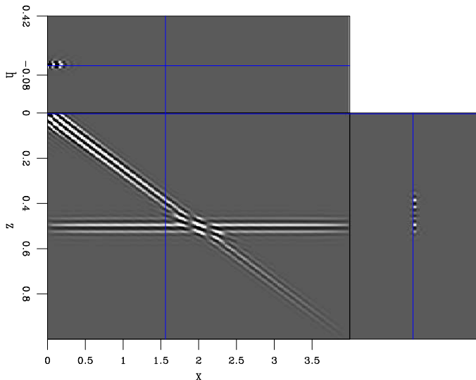
Figure 7: ] Areal shot migration using time-windowed imaging condition of 51 sets, each set containing the summation of areal shots initiated at every 51 th SODCIG. Compare with Figure 4. Original figure was substituted. [ER] armig51T [ER]
