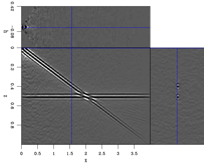
Figure 14: ] Areal shot migration of randomly encoded data. 4 groups of 11 sets of (z_\xi, x_\xi, \omega) -randomly encoded areal data were migrated. Compare with Figures 6, 12 and 13. Original figure was substituted. [ER] arm11phz4 [ER]
