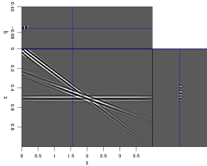
Figure 4: ] Areal shot migration of 51 sets, each set containing the summation of areal shots initiated at every 51 th SODCIG. Original figure was substituted.[ER] armig51W [ER]
