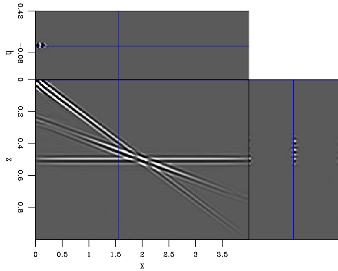
Figure 5: ] Areal shot migration of 41 sets, each set containing the summation of areal shots initiated at every 41 th SODCIG. Original figure was substituted.[ER] armig41W [ER]
