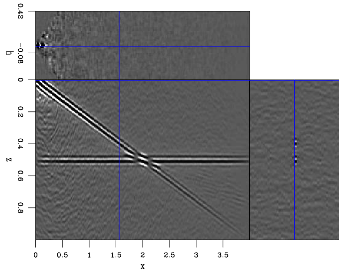
Figure 13: ] Areal shot migration of randomly encoded data. 11 sets of (z_\xi, x_\xi, \omega) -randomly encoded areal data were migrated. Compare with Figure 6. Original figure was substituted. [ER] arm11phz [ER]
