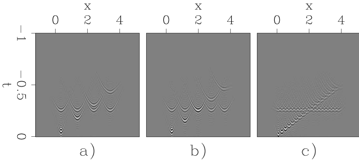
Figure 2: ] Sets of areal sources computed with different distances between SODCIGs. a) 51 traces; b) 41 traces; and c) 11 traces. [ER] arsource [ER]
