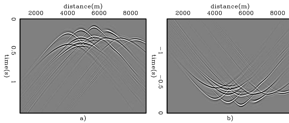
Figure 9: PERM wavefields for the Marmousi example: a) Receiver wavefield. b) Source wavefield.
