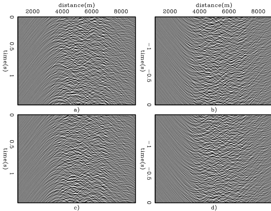
Figure 11: ISPEWs from different random realizations initiated at the same SODCIGs for the Marmousi example: a,c) Receiver wavefields. b,d) Source wavefields.
