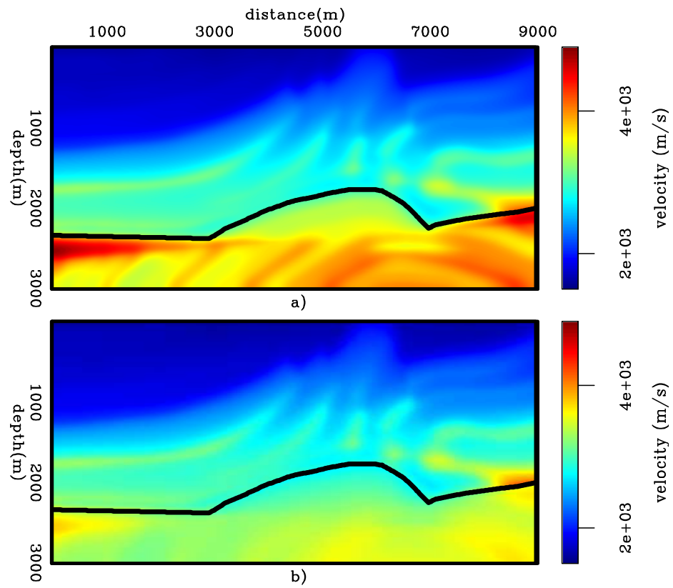
Figure 6: Velocity models for the Marmousi example: a) Smooth velocity model used to model the Born data. b) Background velocity model used to migrate the Born data, and to model and migrate PERM data.
