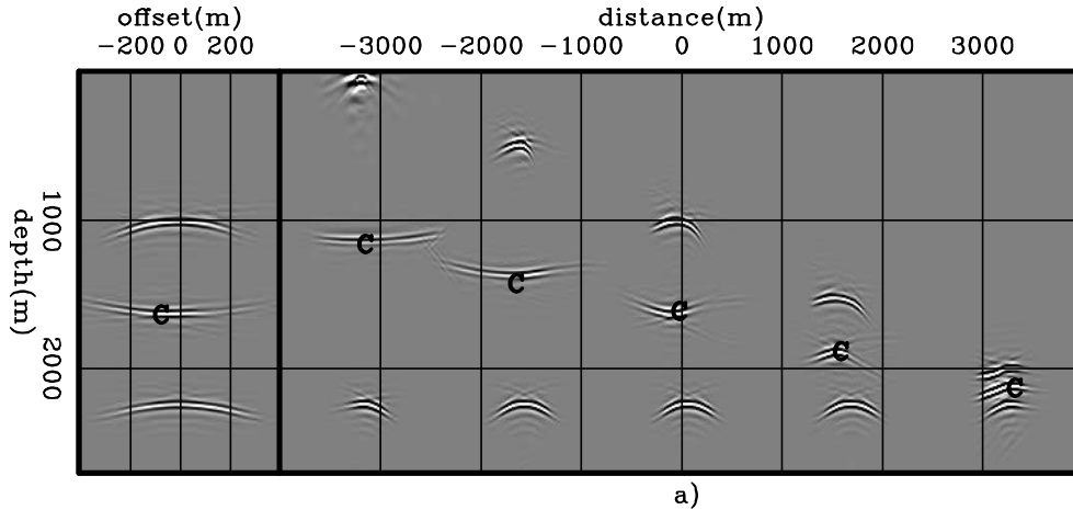
Figure 1: Areal-shot migration of PERM data synthesized from a set of SODCIGs selected with sampling period of 163. The two reflectors are simultaneously injected to the model. Notice the reflector crosstalk, labeled with ‘C’, resulting from the cross-correlation of the wavefields from the horizontal reflector with that from the dipping reflector.
