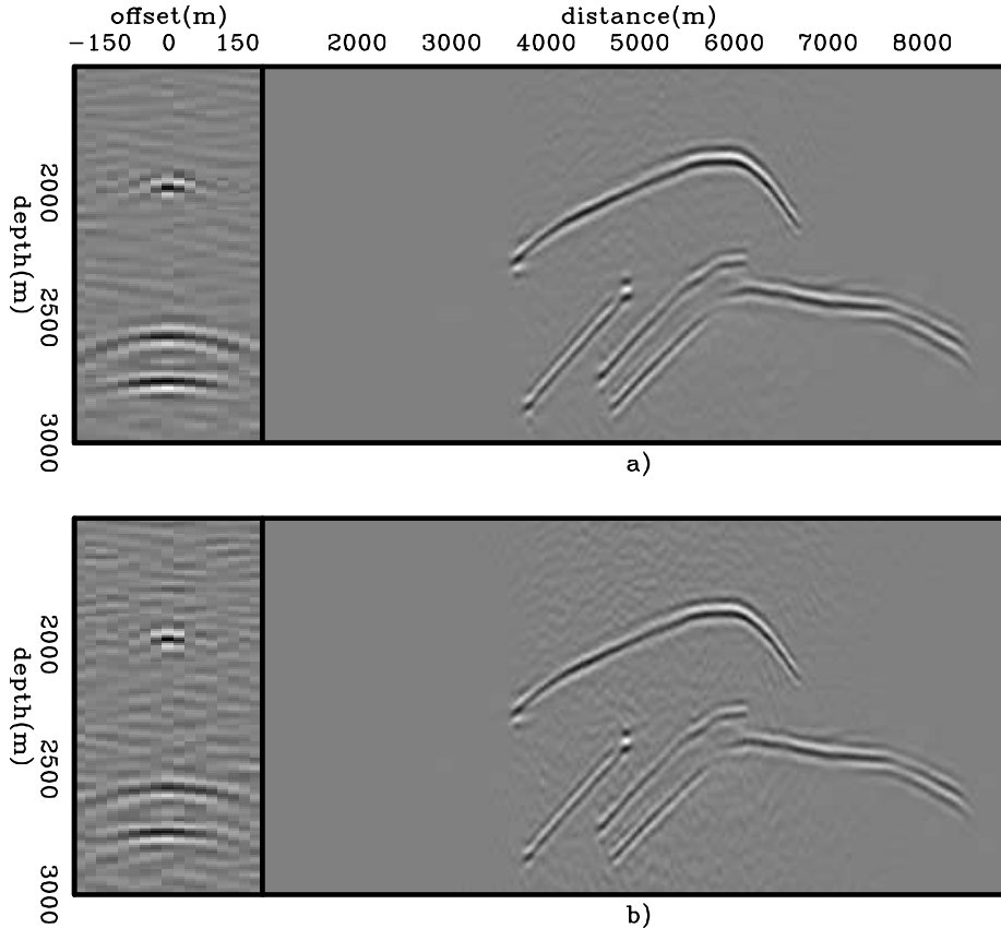
Figure 12: Pre-stack images computed with: a) Four random realizations of ISPEWs, and b) a single random realization.
