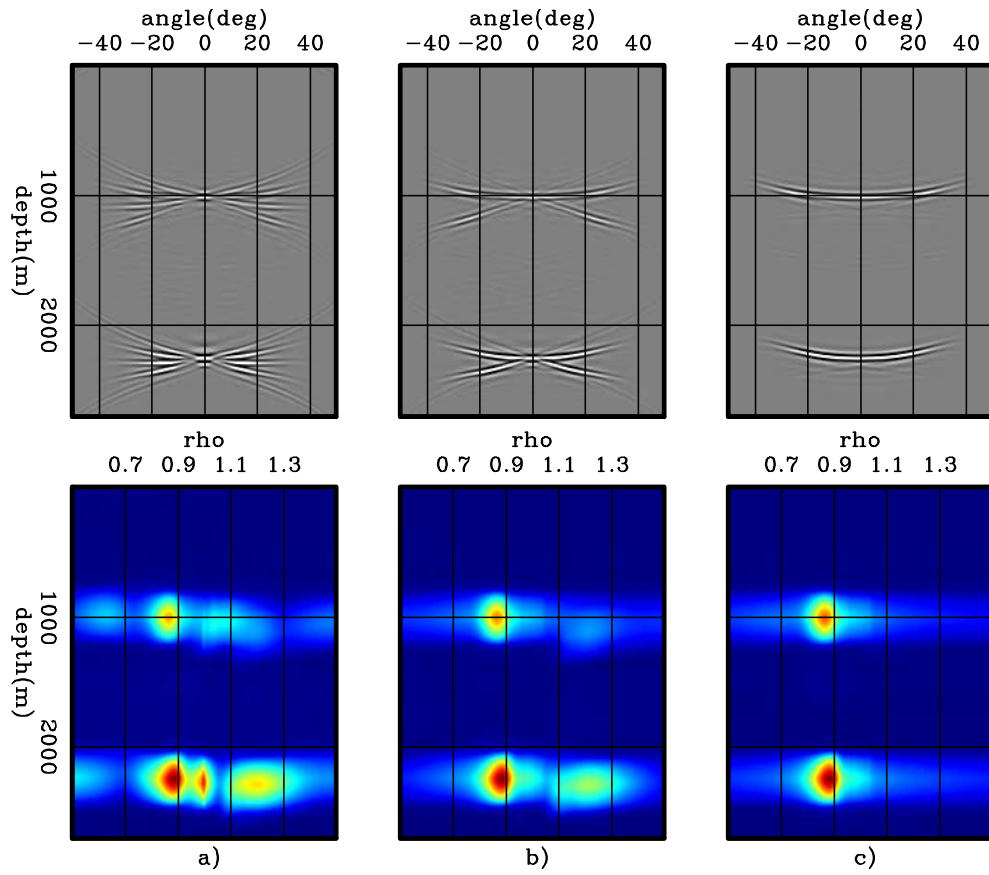
Figure 4: ADCIGs (top) and \rho -panels (bottom) corresponding to images computed by wavefields modeled with sampling period of: a) 41, b) 81, and c) 163. Velocity information has been destroyed by the crosstalk in a) and b).
