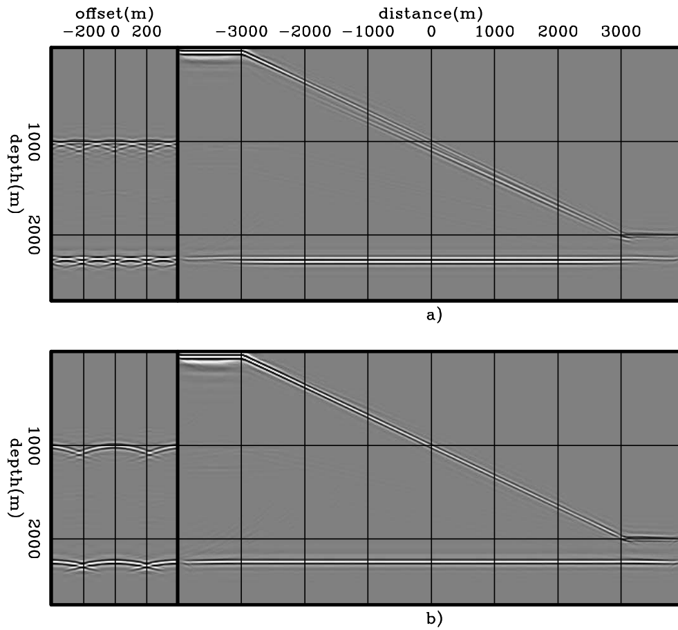
Figure 3: Areal-shot migration of PERM data synthesized from sets of SODCIGs selected with sampling period of: a) 41 and, b) 81.
