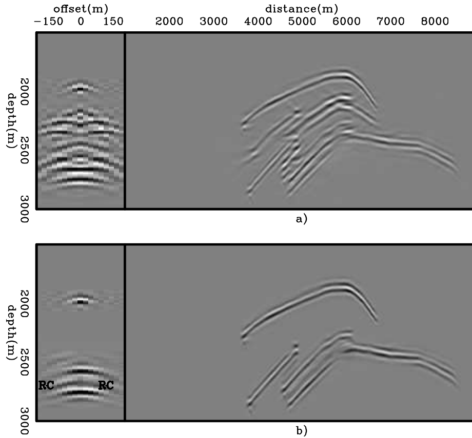
Figure 10: Pre-stack image computed with PERM wavefields and background velocity model using: a) the conventional imaging condition (equation ??), and b) the time-windowed imaging condition (equation 2). Reflector crosstalk is avoided when reflectors are sufficiently separated. However, some residual crosstalk is still present (RC). Notice the phase difference of the PERM image due to the squaring of the wavelet when compared to the windowed reflectors of Figure 7b.
