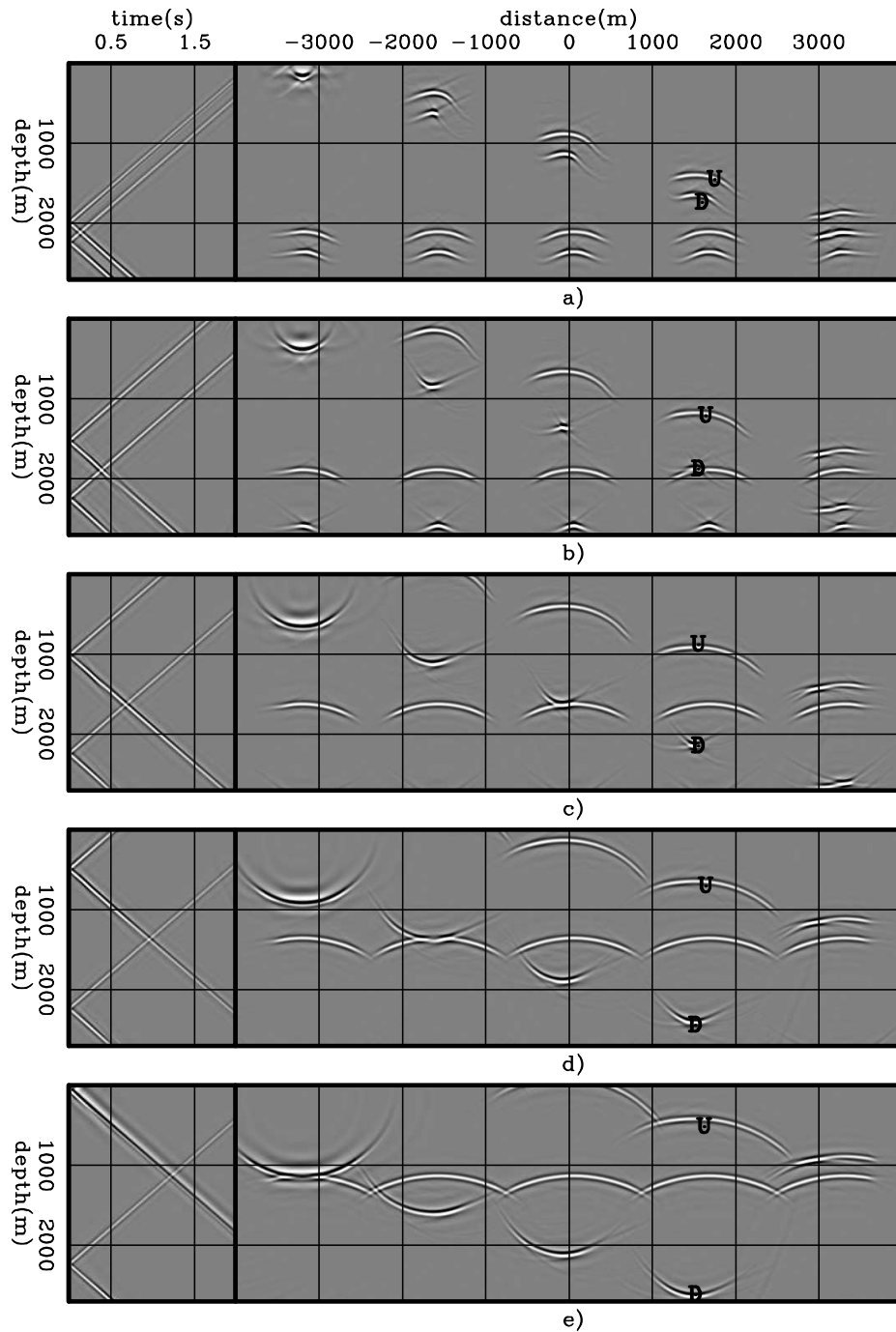
Figure 2: Snapshots of propagation of wavefields used to compute the image of Figure 1. Wavefields are labeled 'D' (Downgoing) for the source wavefield and 'U' (Upgoing) for the receiver wavefield. The panels on the left are selected at horizontal positions where the crosstalk occurs in Figure 1. The panels on the right are taken at the propagation time when the wavefields cross on the left panel.
