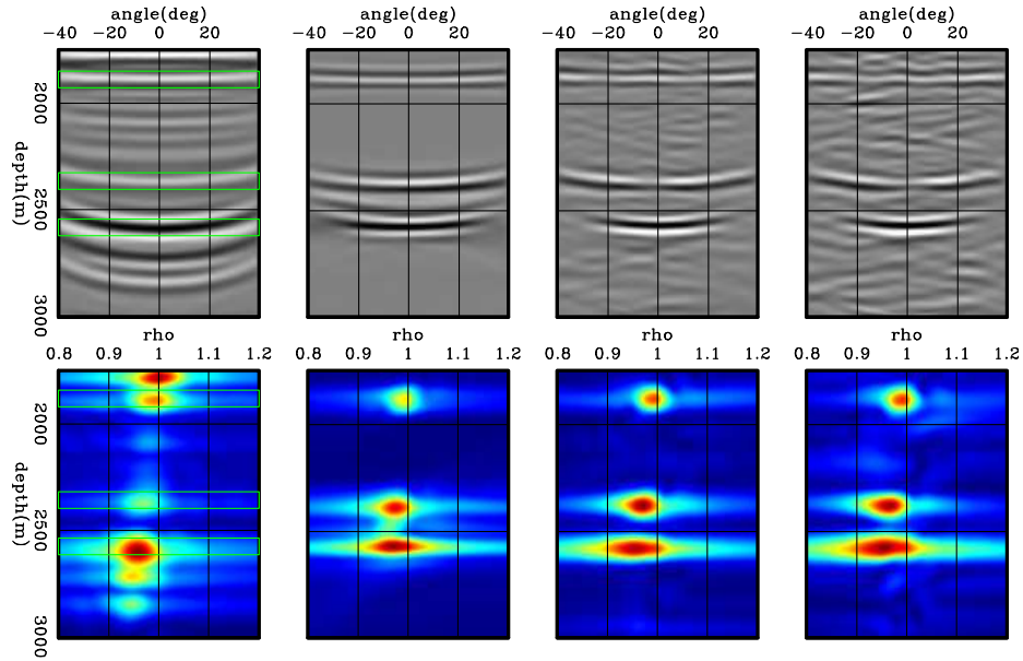
Figure 13: ADCIGs (top) and \rho -panels (bottom) corresponding to images computed by: a) Shot-profile migration of 360 shot gathers, b) areal-shot migration of 35 PERM wavefields using the time-windowed imaging condition, c) areal-shot migration of 44 ISPEWs corresponding to four random realizations, and d) areal-shot migration of 11 ISPEWs corresponding to a single random realization. The moveout information is basically the same.
