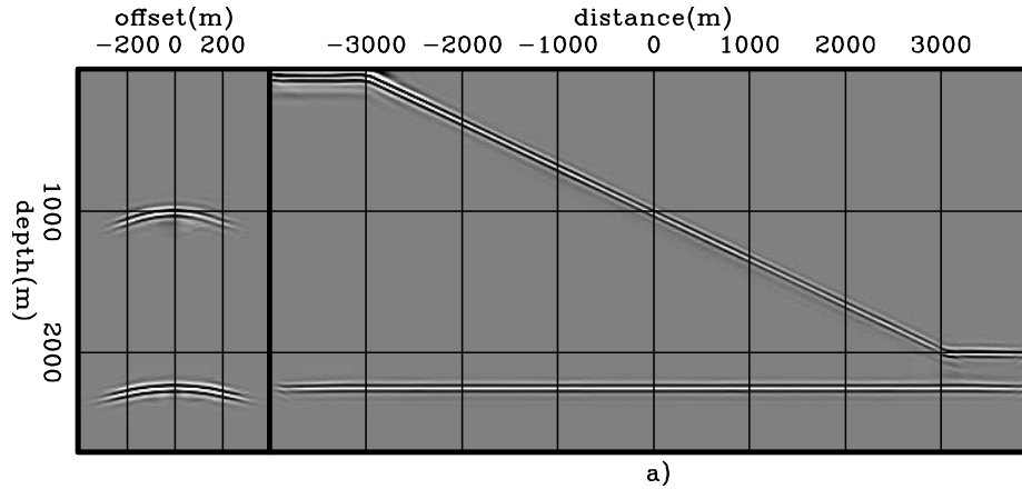
Figure 5: Areal-shot migration using the time-windowed imaging condition (equation 2). The reflector crosstalk is completely eliminated.
