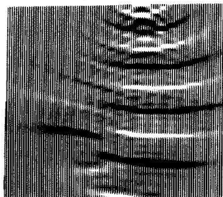
Four frequency reconstruction
