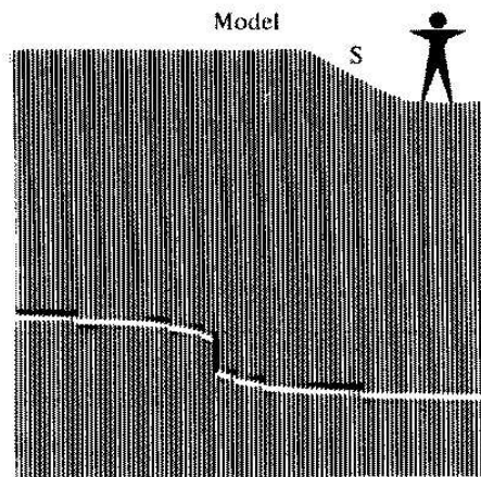
Four frequency reconstruction
