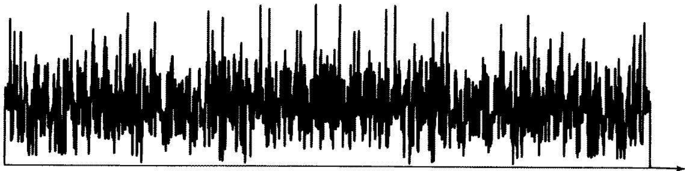
Amplitude spectrum of white noise sample
