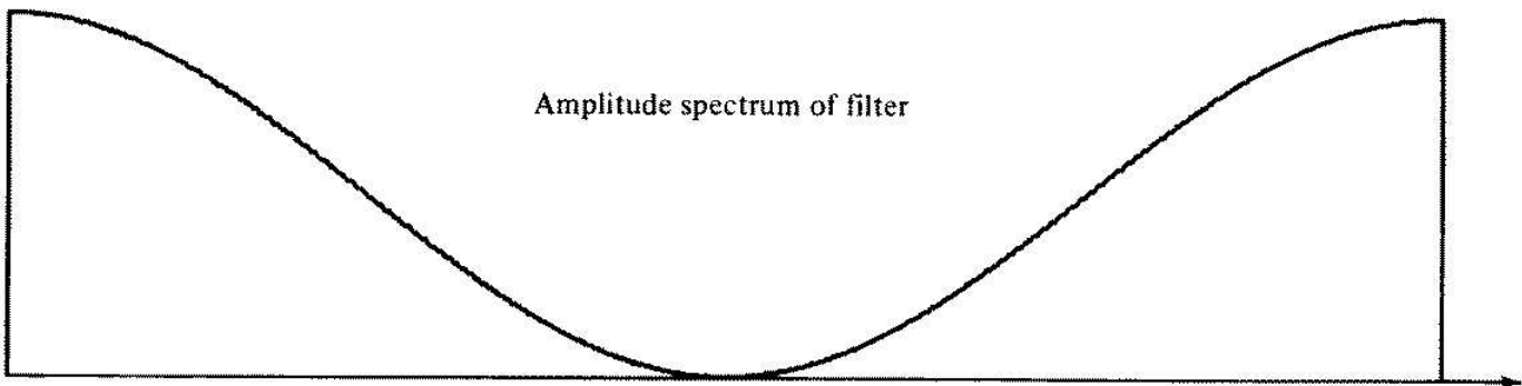
Unsmoothed power spectral estimate of data sample
