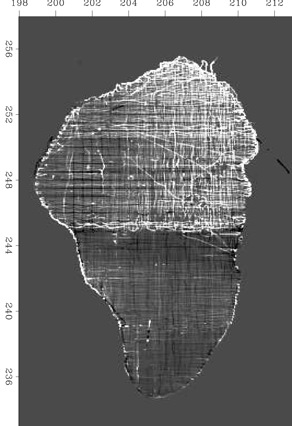
Data drift in model space
