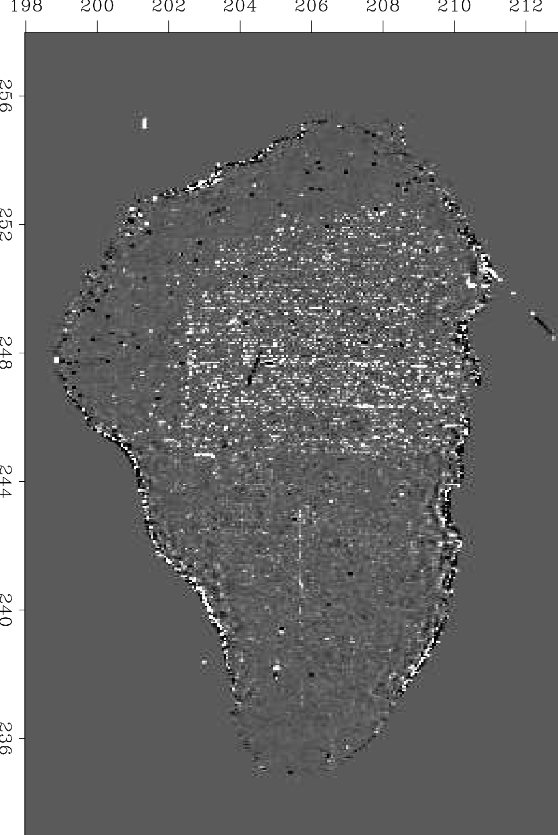
Data residual in model space
