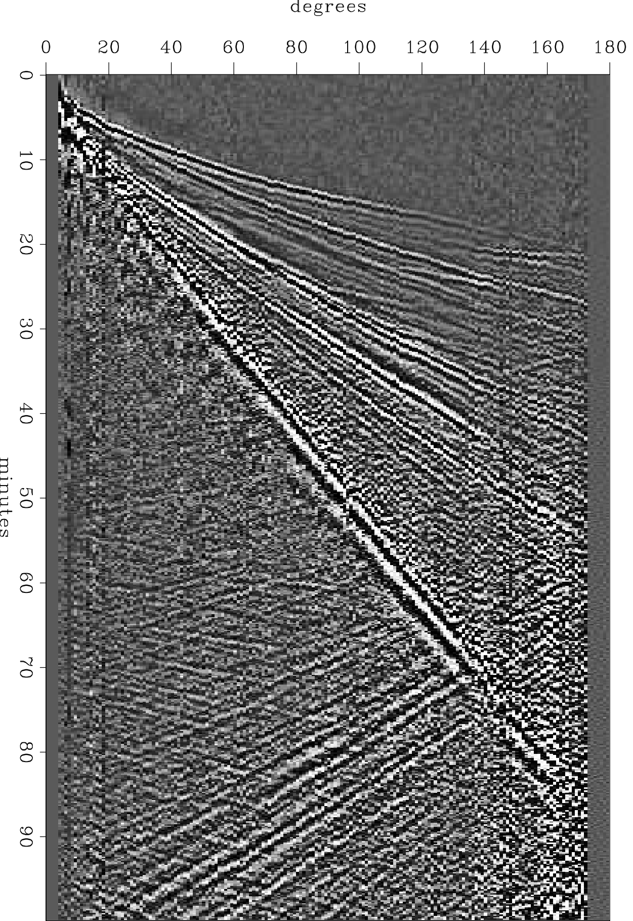
stack (gpow=.5)
