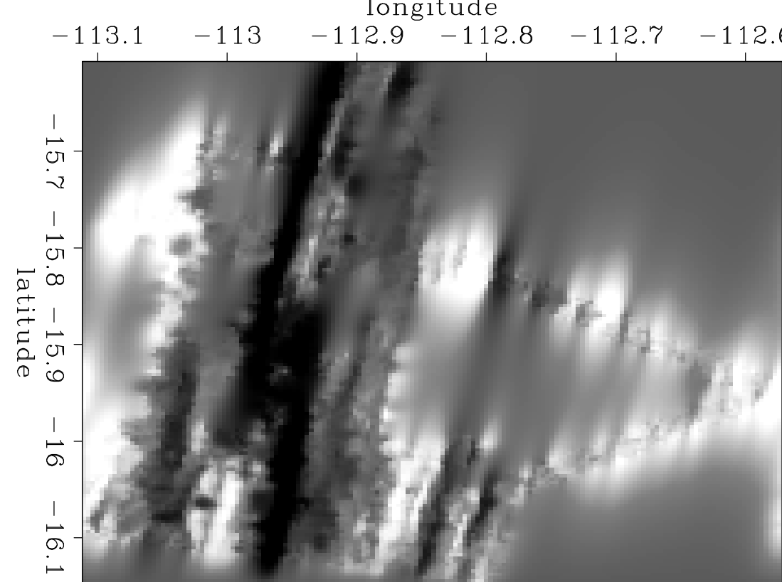
PEF Interpolation
