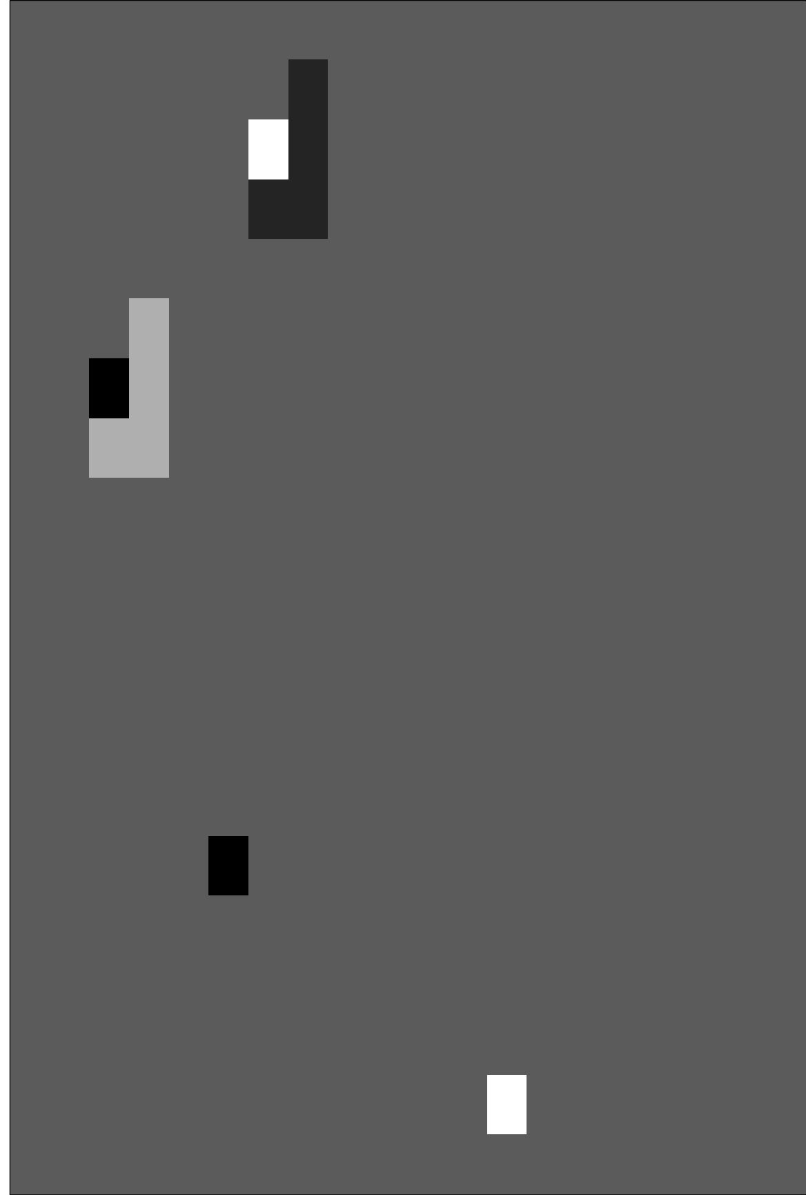
((\text{input}/\text{filter})/\text{filter}')\text{filter}'\text{filter}
