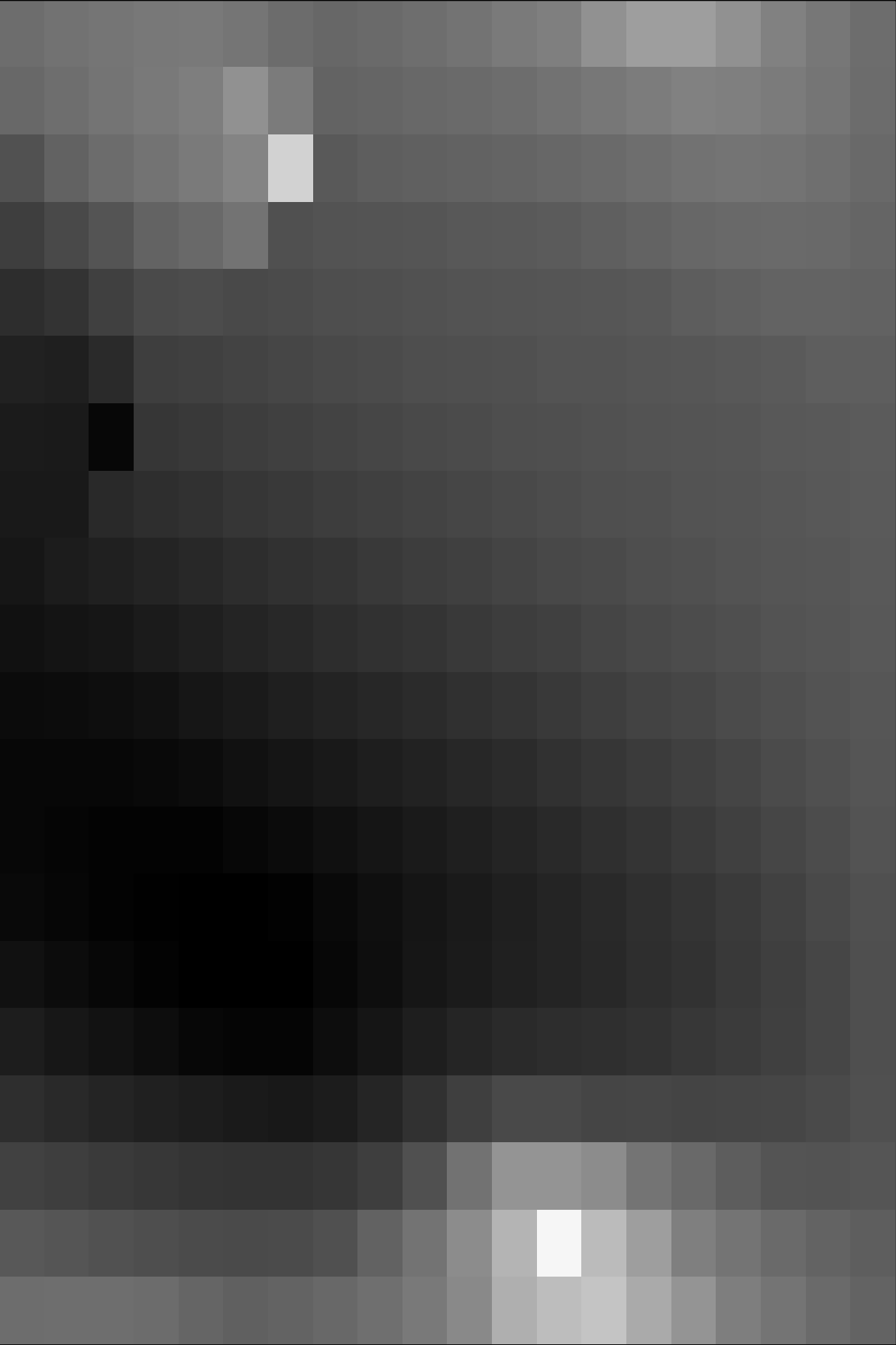
(\text{input}/\text{filter})/\text{filter}'
