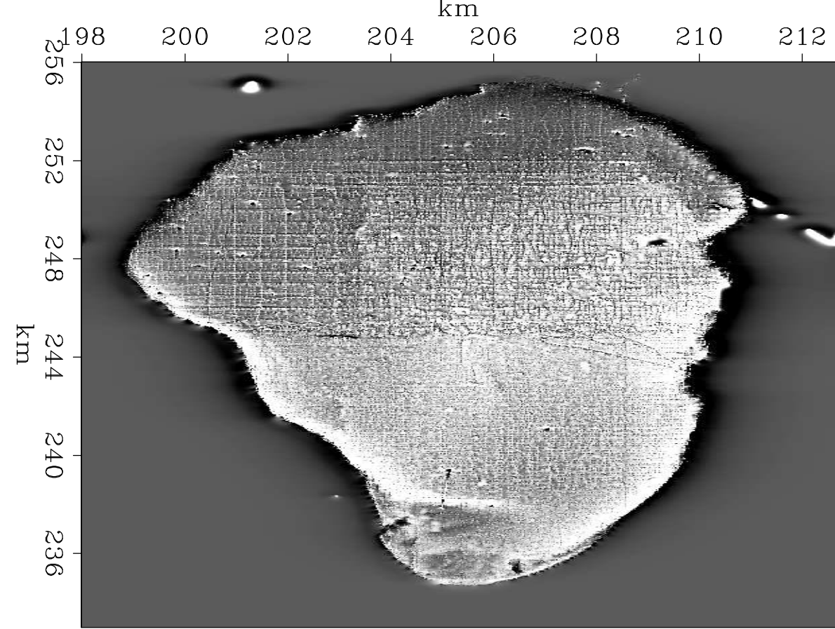
Filled and helix deriv
