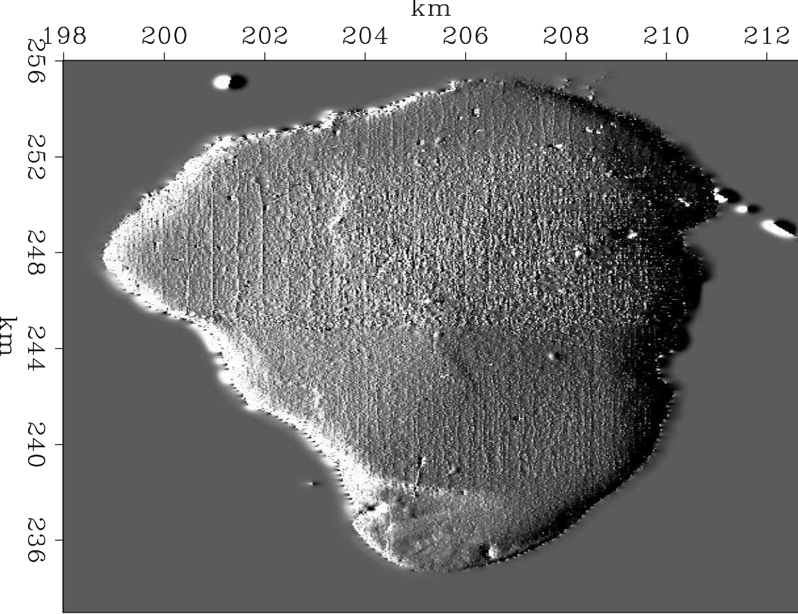
Filled and d/dx
