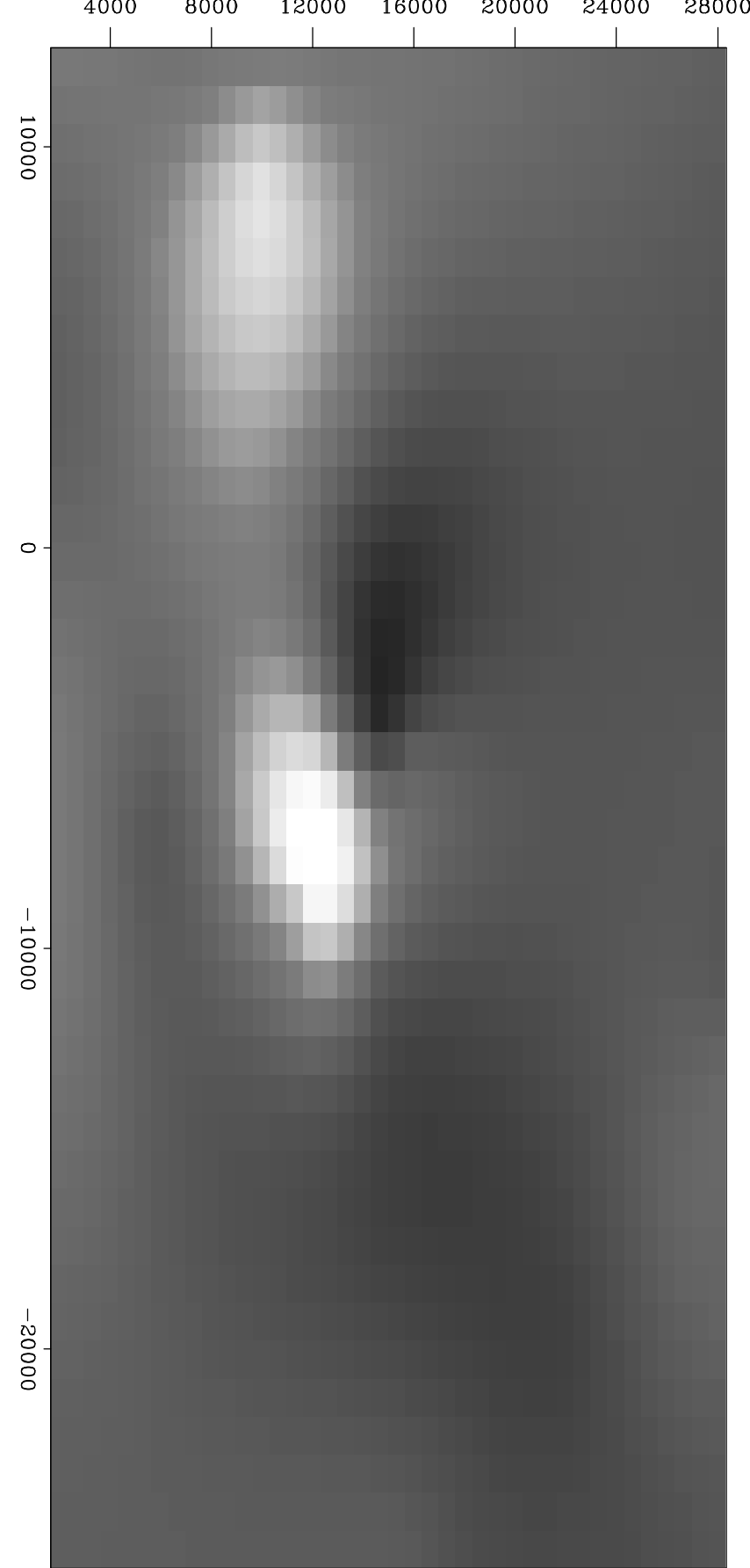
Laplacian_map - Seismic
