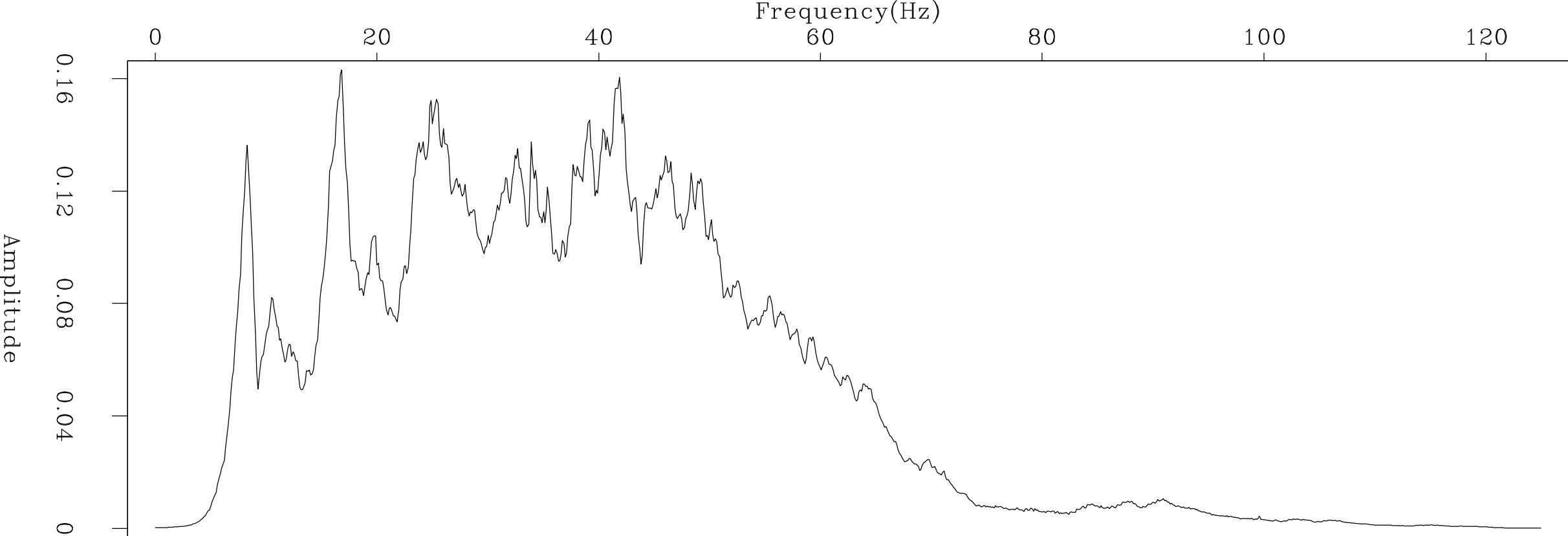
Spectrum Data
