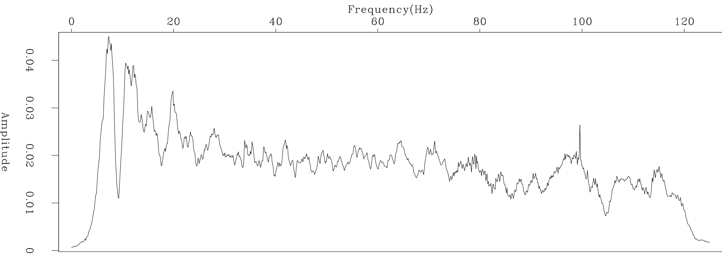
Spectrum PEF*Data
