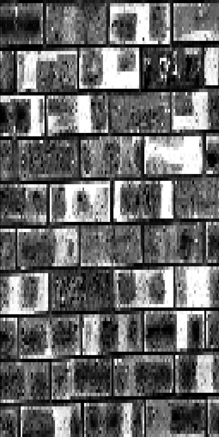
Training Image
