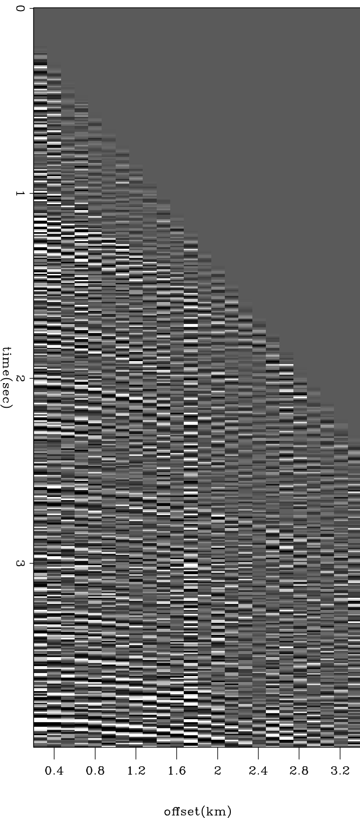
CMP Gather
