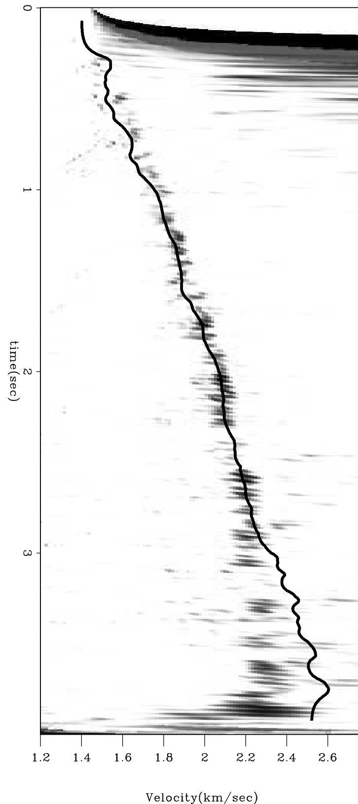
Semblance Scan
