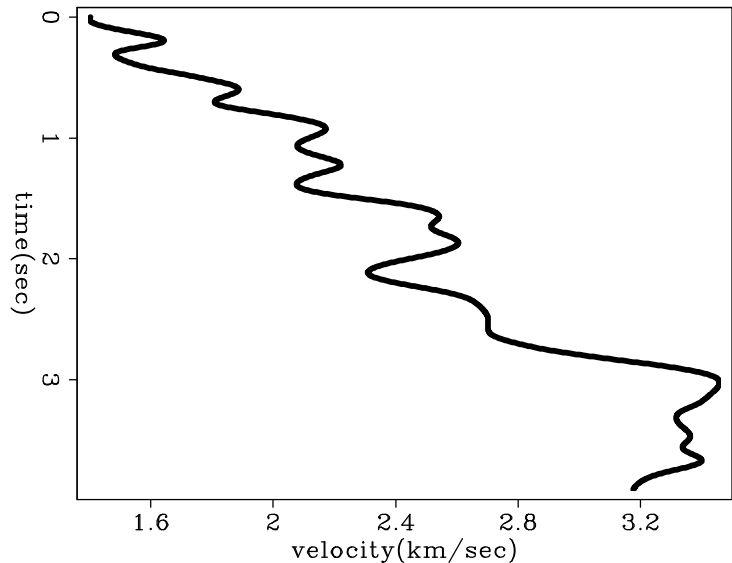
Interval velocity
