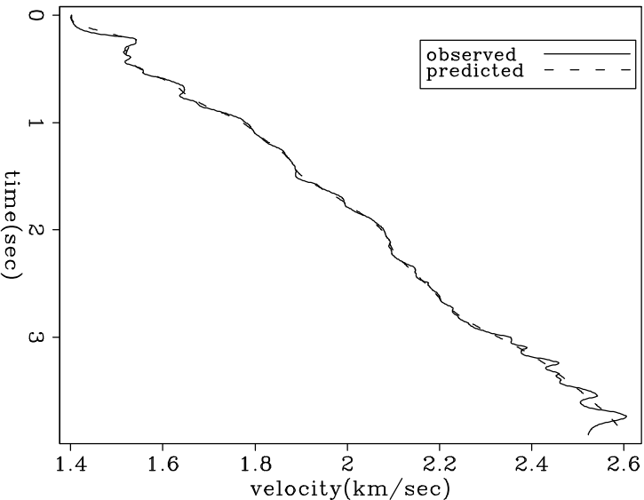
RMS Velocity
