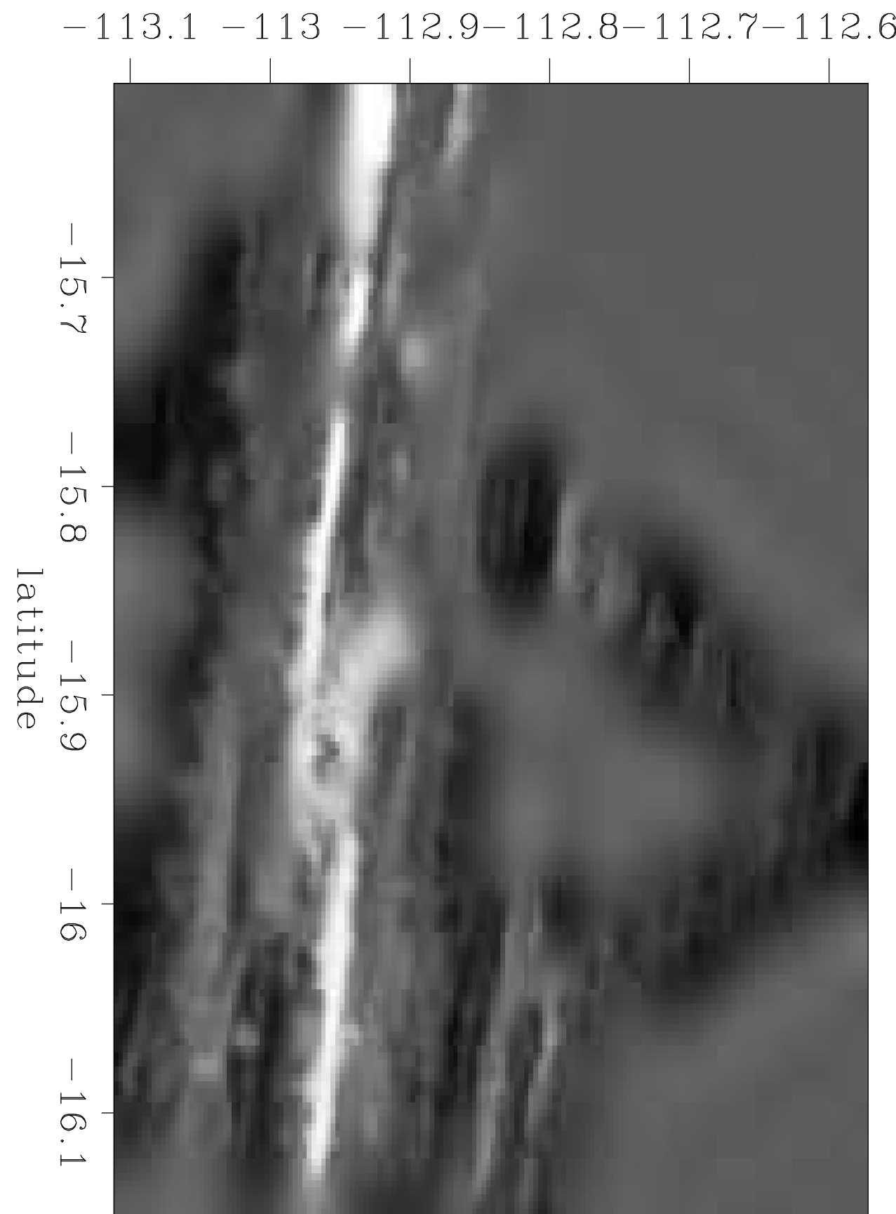
April_18_Laplacian
