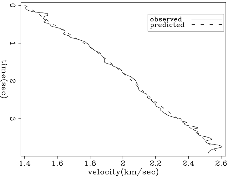
RMS Velocity
