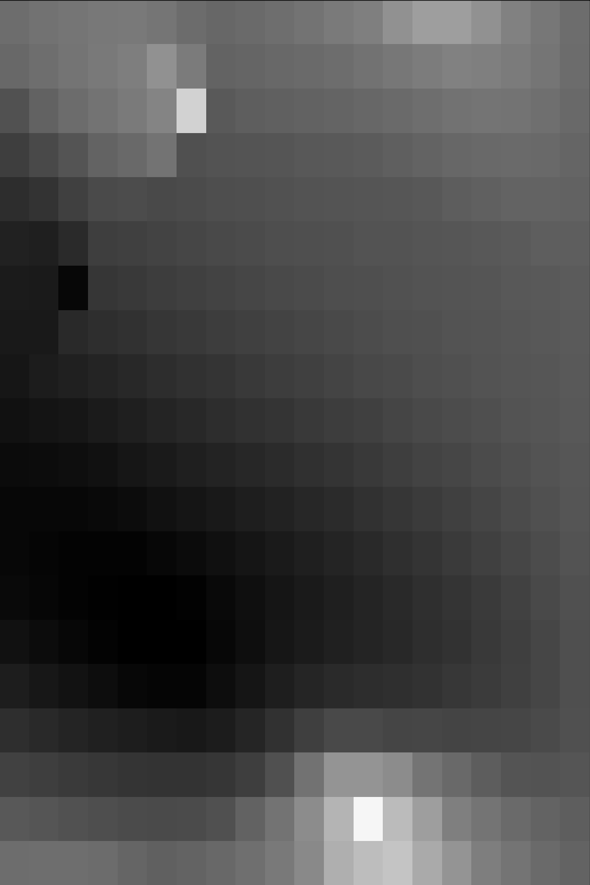
(\text{input}/\text{filter})/\text{filter}'
