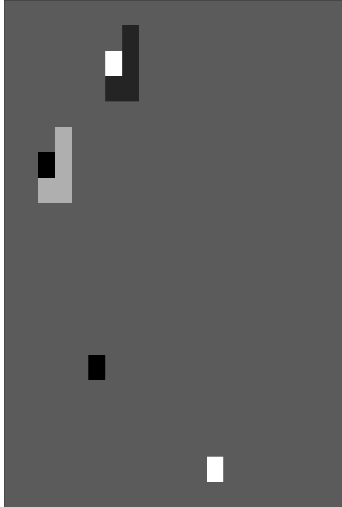
((\text{input}/\text{filter})/\text{filter}')\text{filter}'\text{filter}
