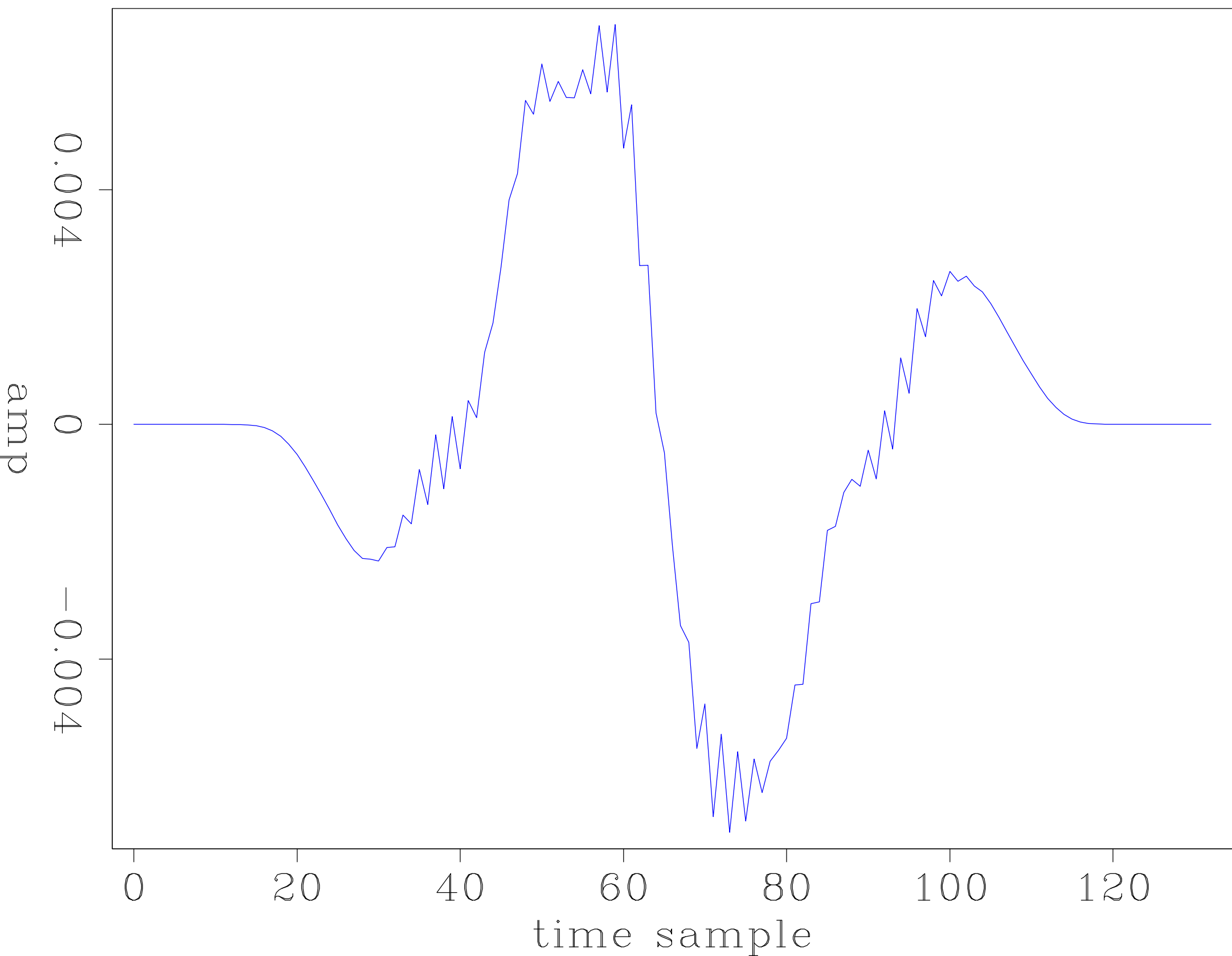
The PEF decon result of Simple (0, -1, 1)
