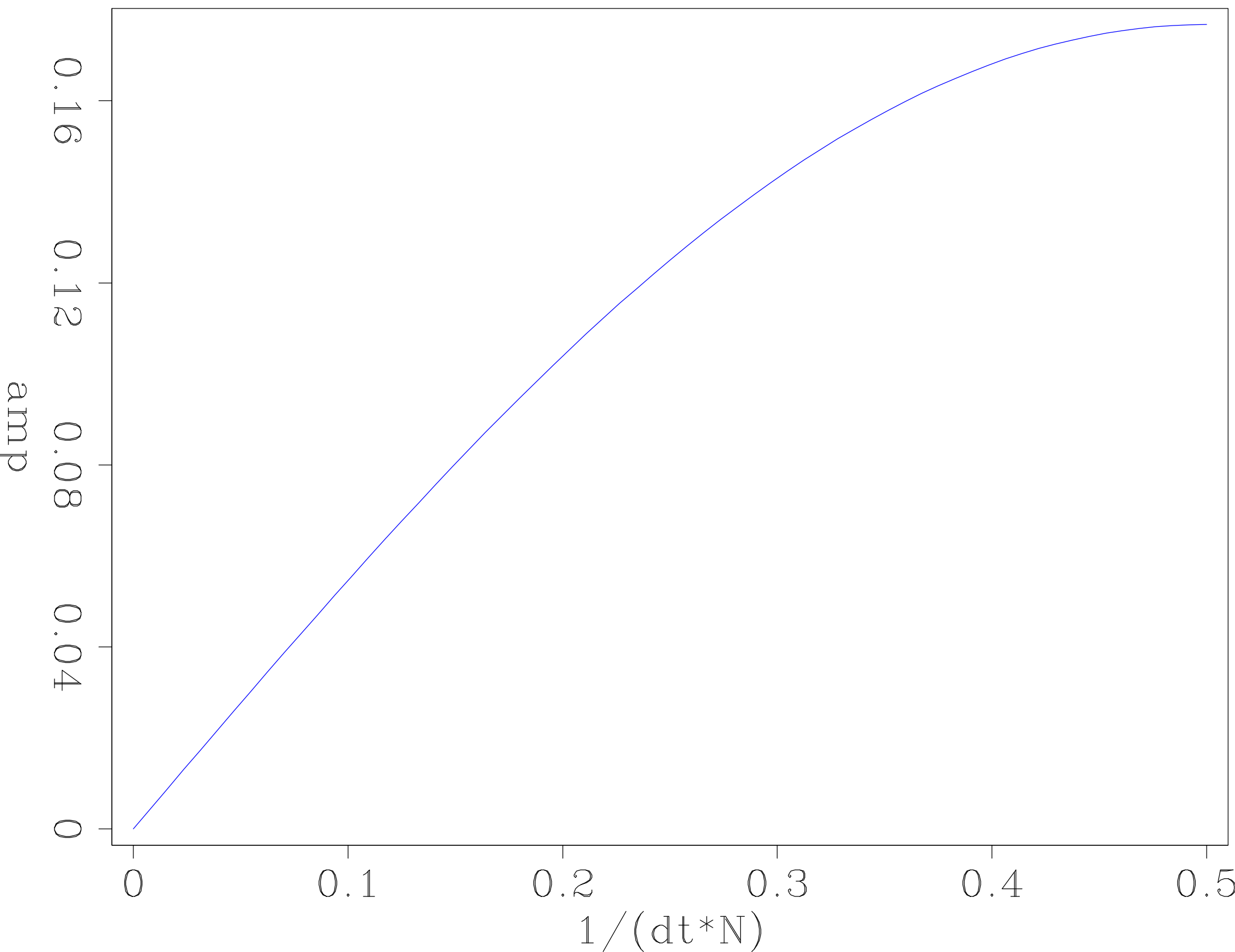
Spectrum of Simple (0, -1, 1)
