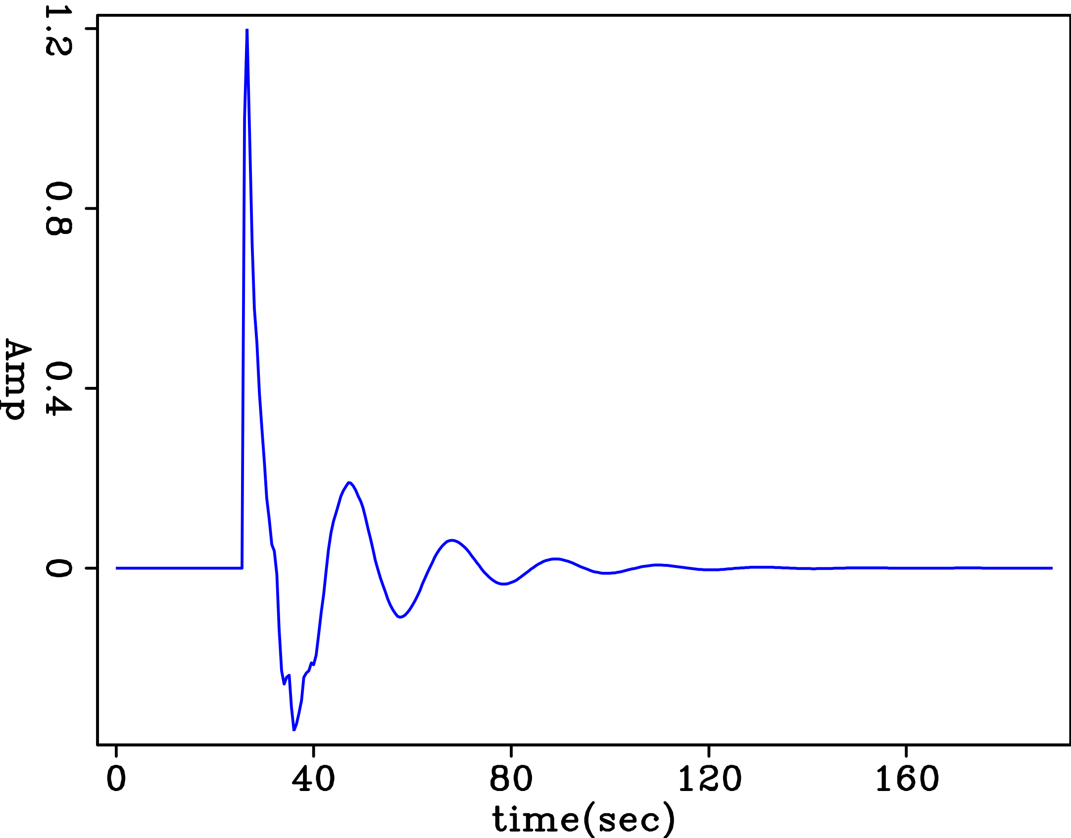
Burg wavelet(dt=0.5sec len=30)
