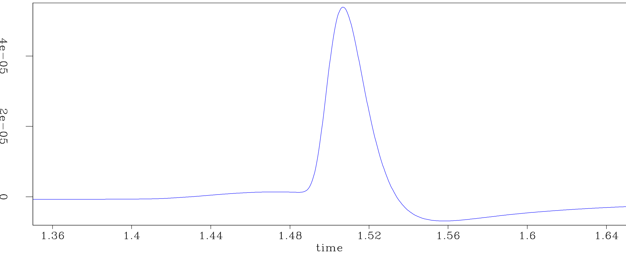
Constant Q response of a spike
