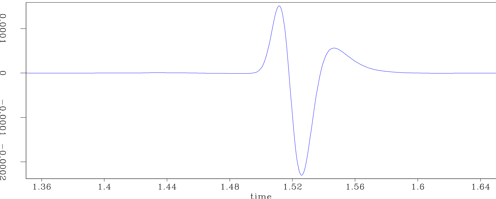
Constant Q response of a Ricker
